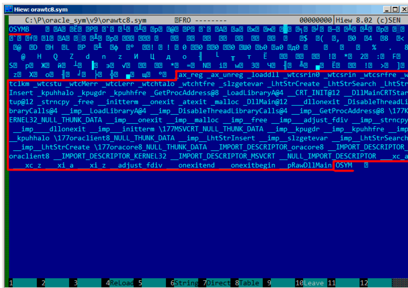
Figure 9.23: OSYM signature and text strings
