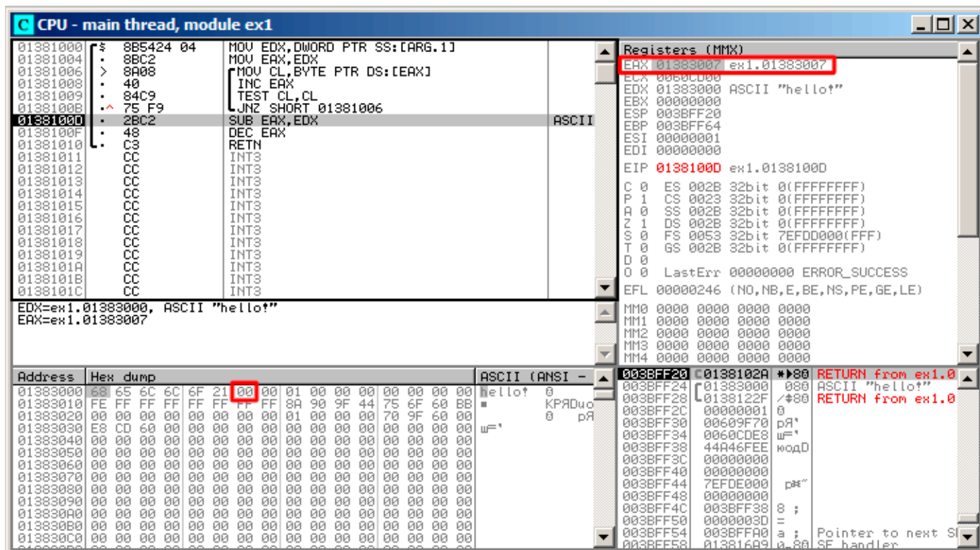
Figure 1.61: OllyDbg: pointers difference to be calculated now
