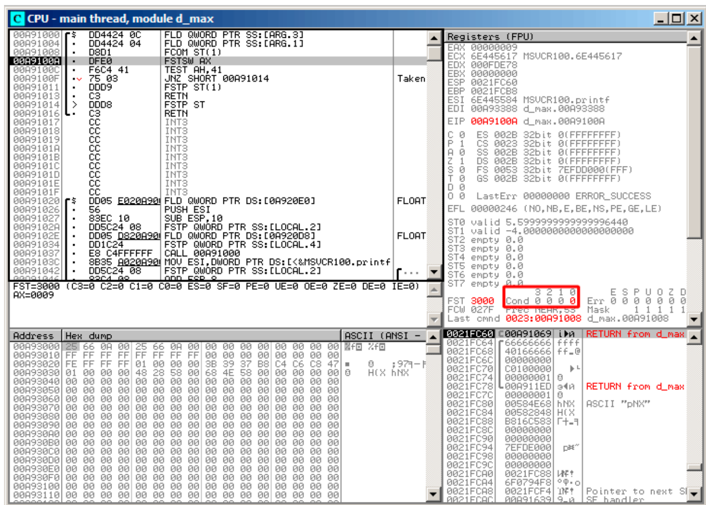
Figure 1.84: OllyDbg: FCOM is finished
