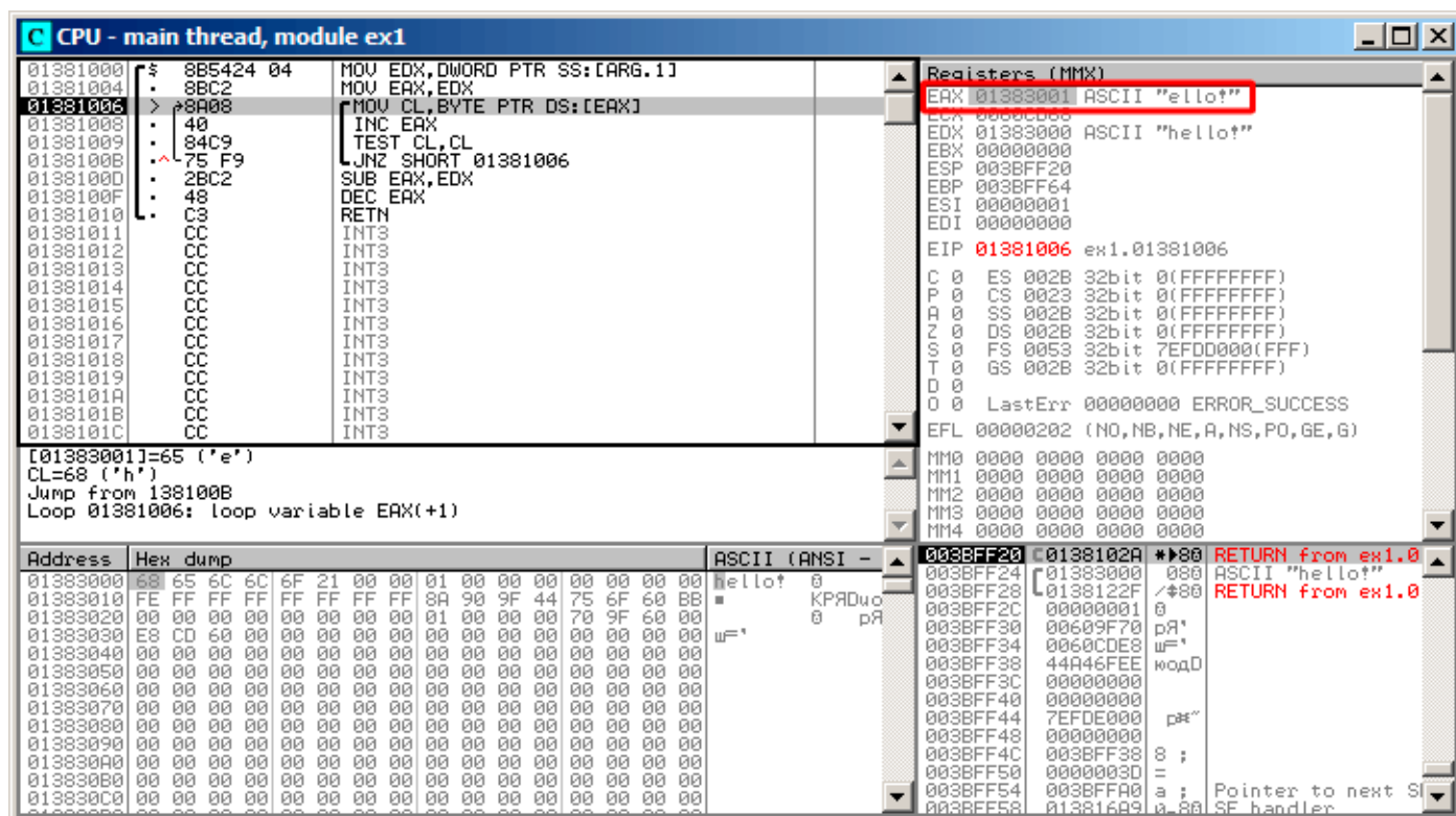
Figure 1.60: OllyDbg: second iteration start
