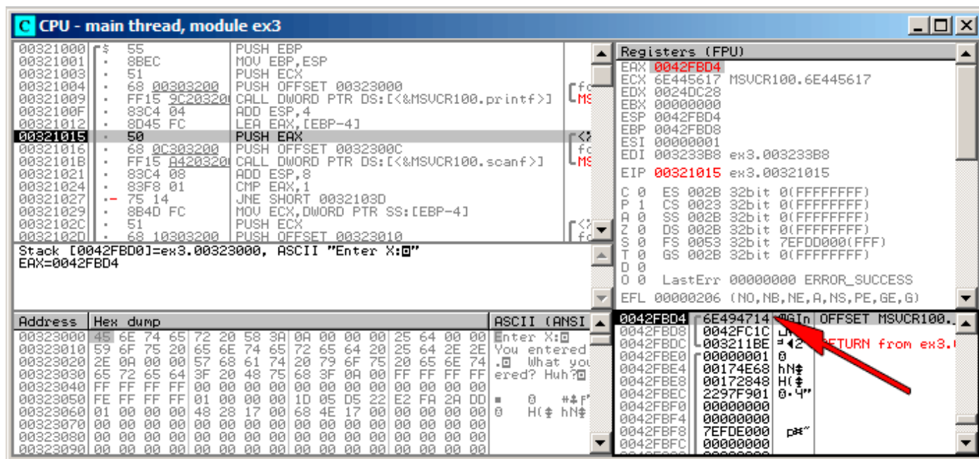
Figure 1.20: OllyDbg: passing variable address into scanf()
