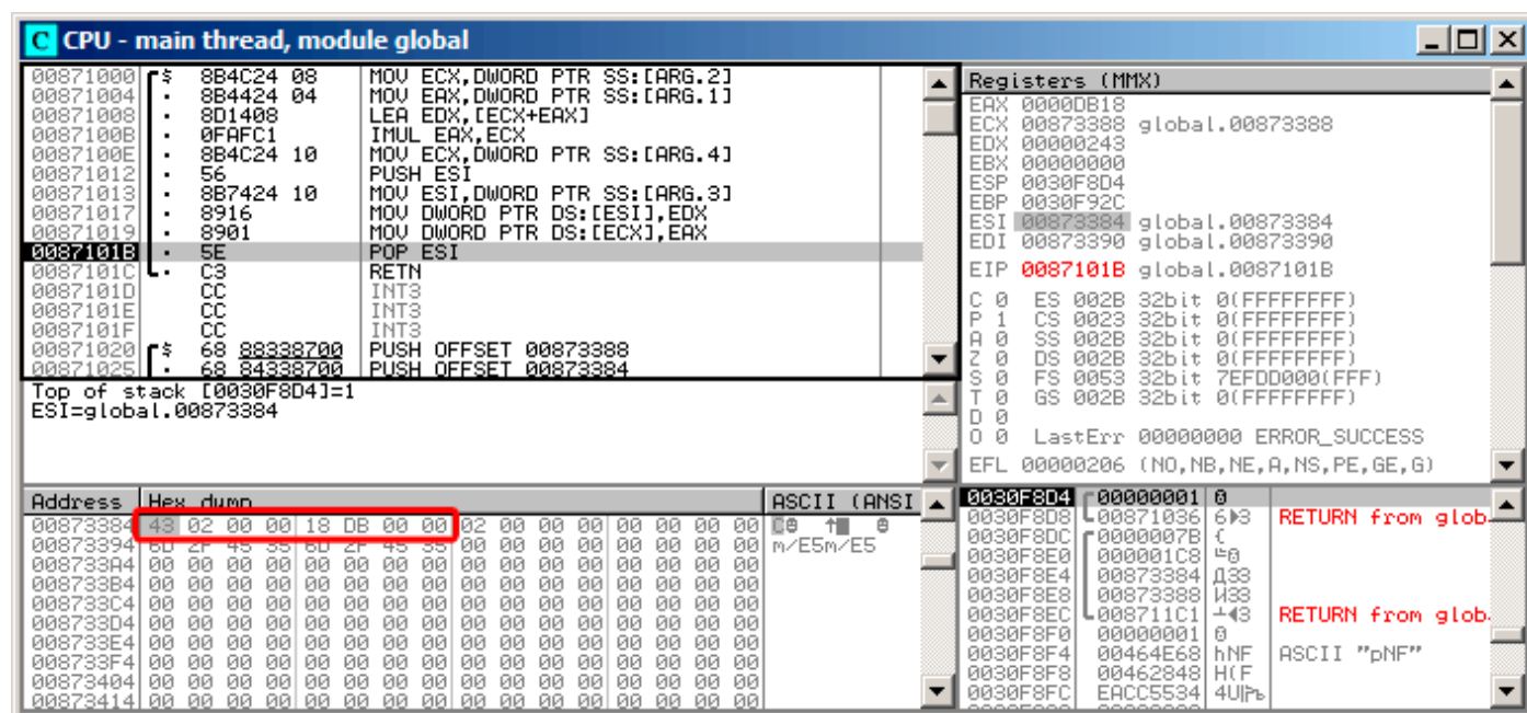
Figure 1.28: OllyDbg: f1() execution completed
