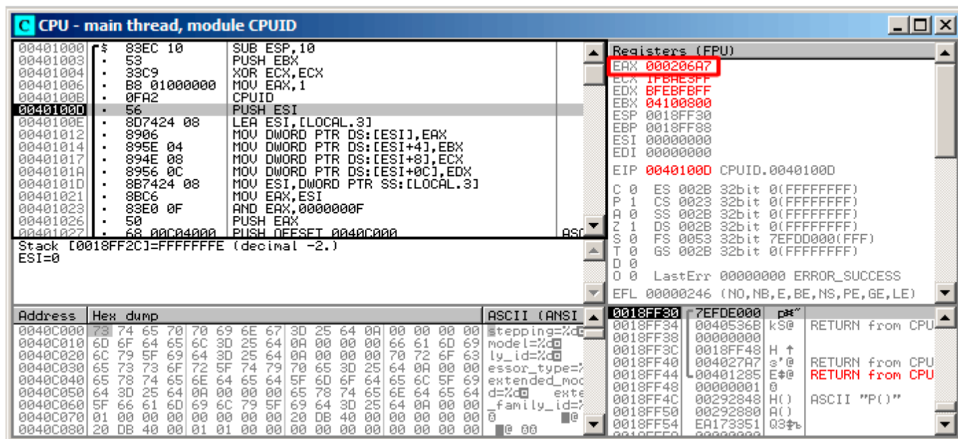
Figure 1.109: OllyDbg: After CPUID execution
