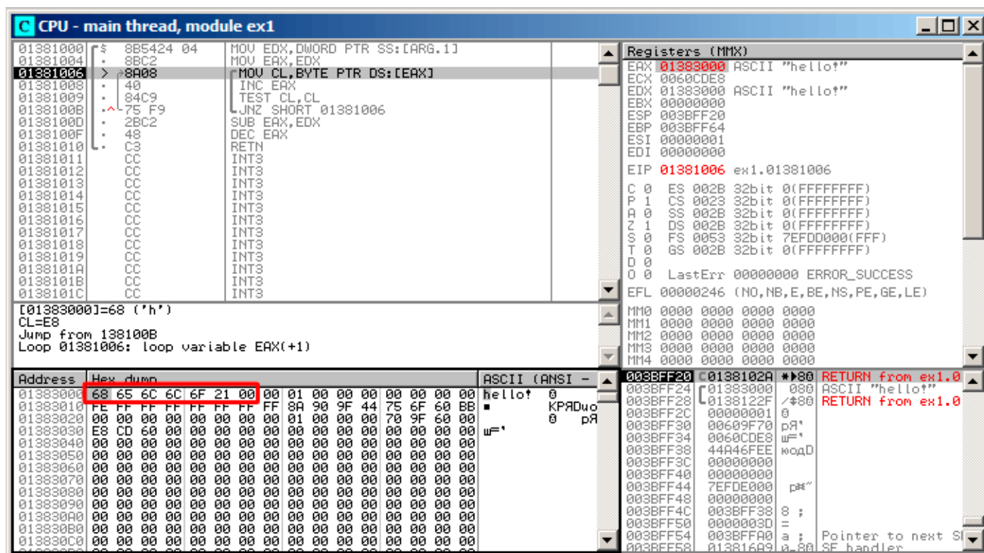
Figure 1.59: OllyDbg: first iteration start
