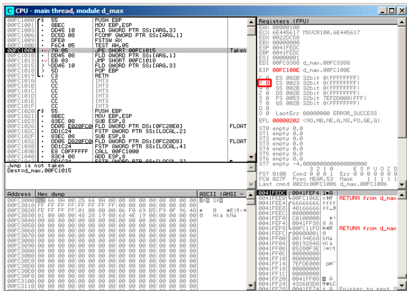
Figure 1.76: OllyDbg: TEST executed
