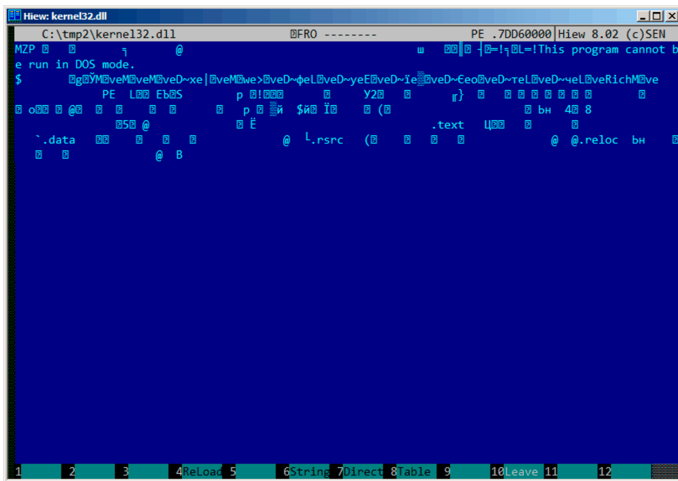
Figure 9.4: Original file
