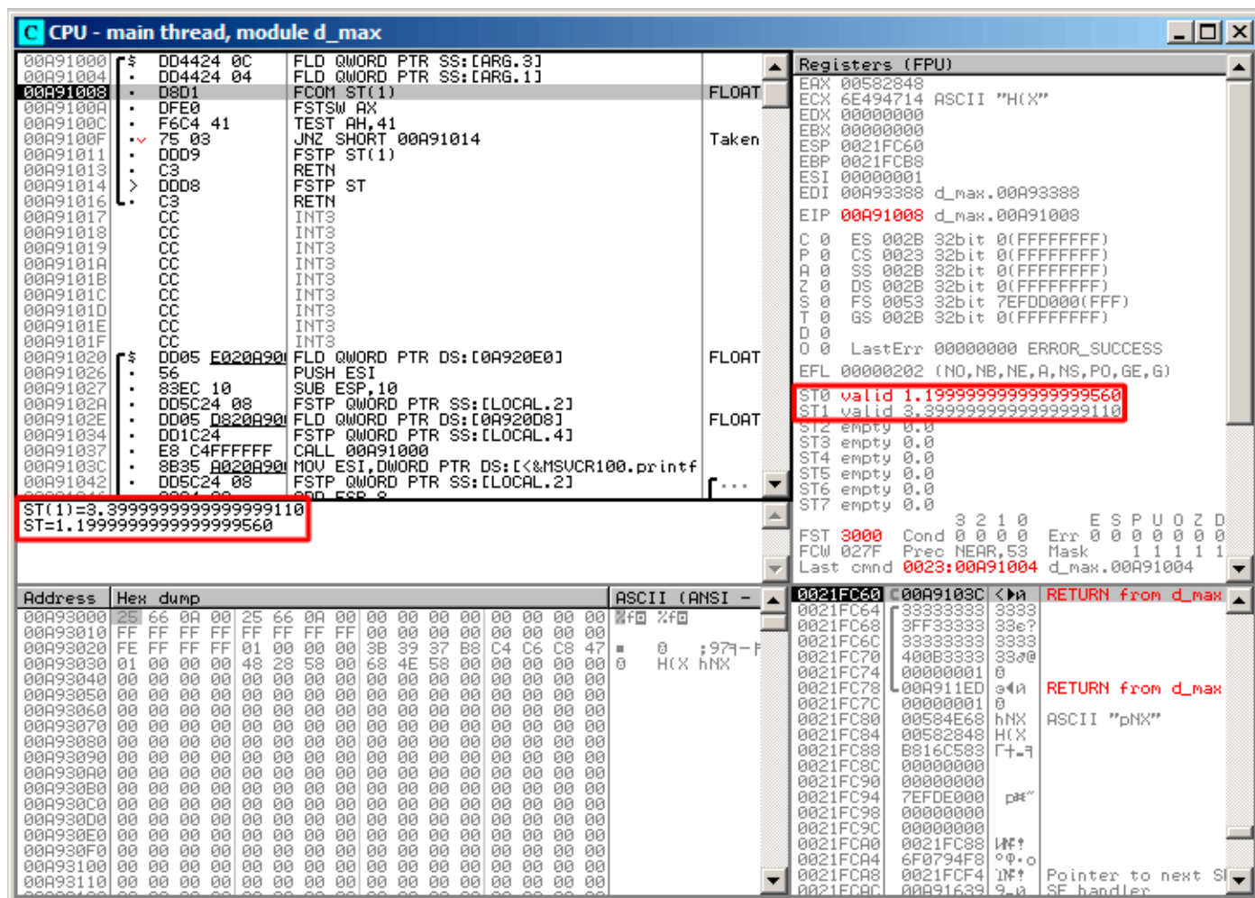
Figure 1.78: OllyDbg: both FLD are executed
