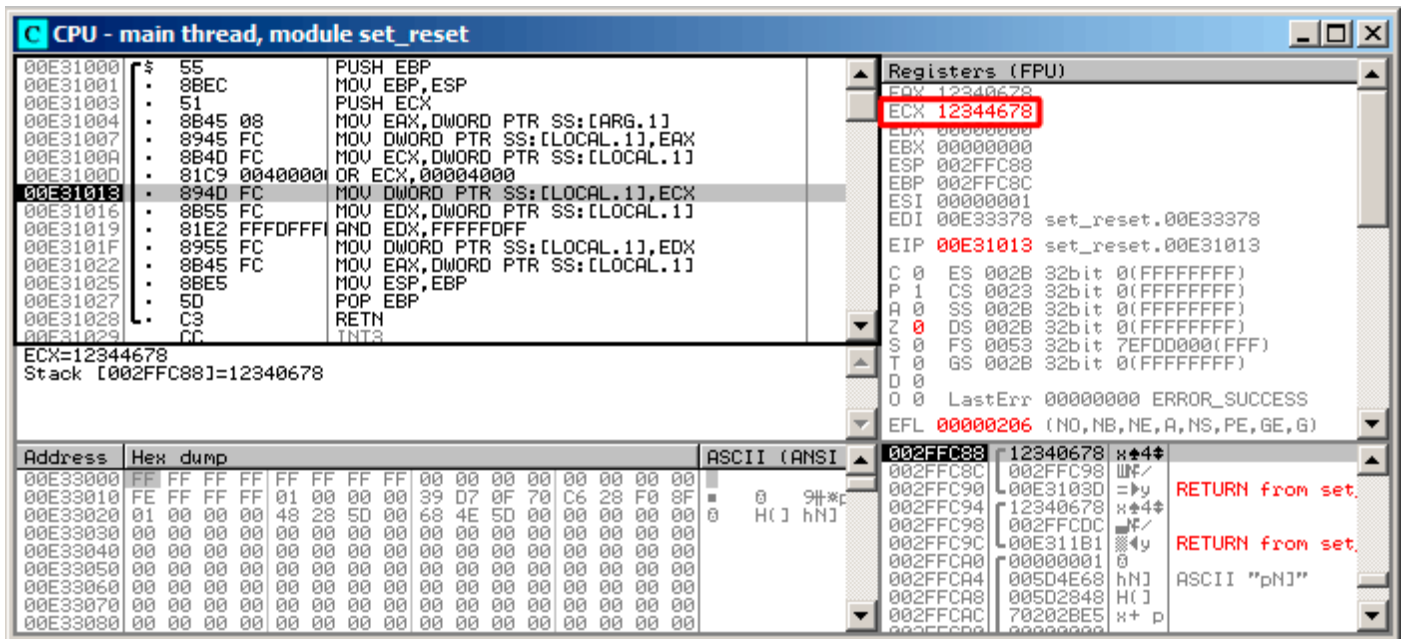
Figure 1.96: OllyDbg: 0R executed
