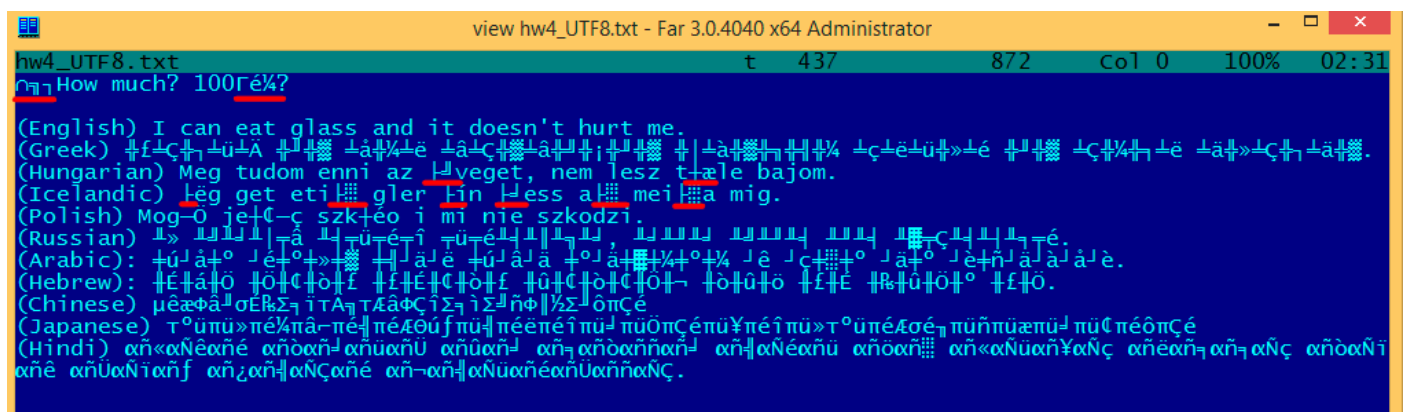
Figure 5.2: FAR: UTF-8
