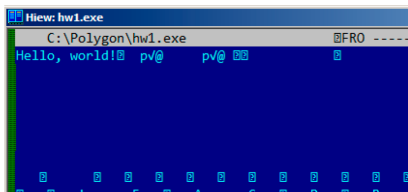
Figure 5.1: Hiew
