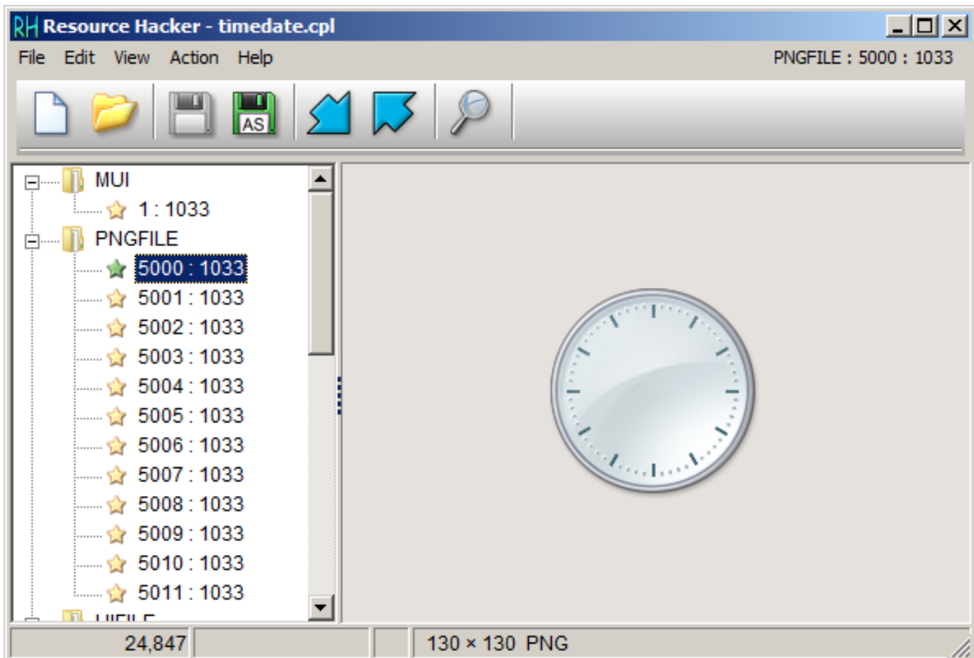
Figure 8.10: Resource Hacker
