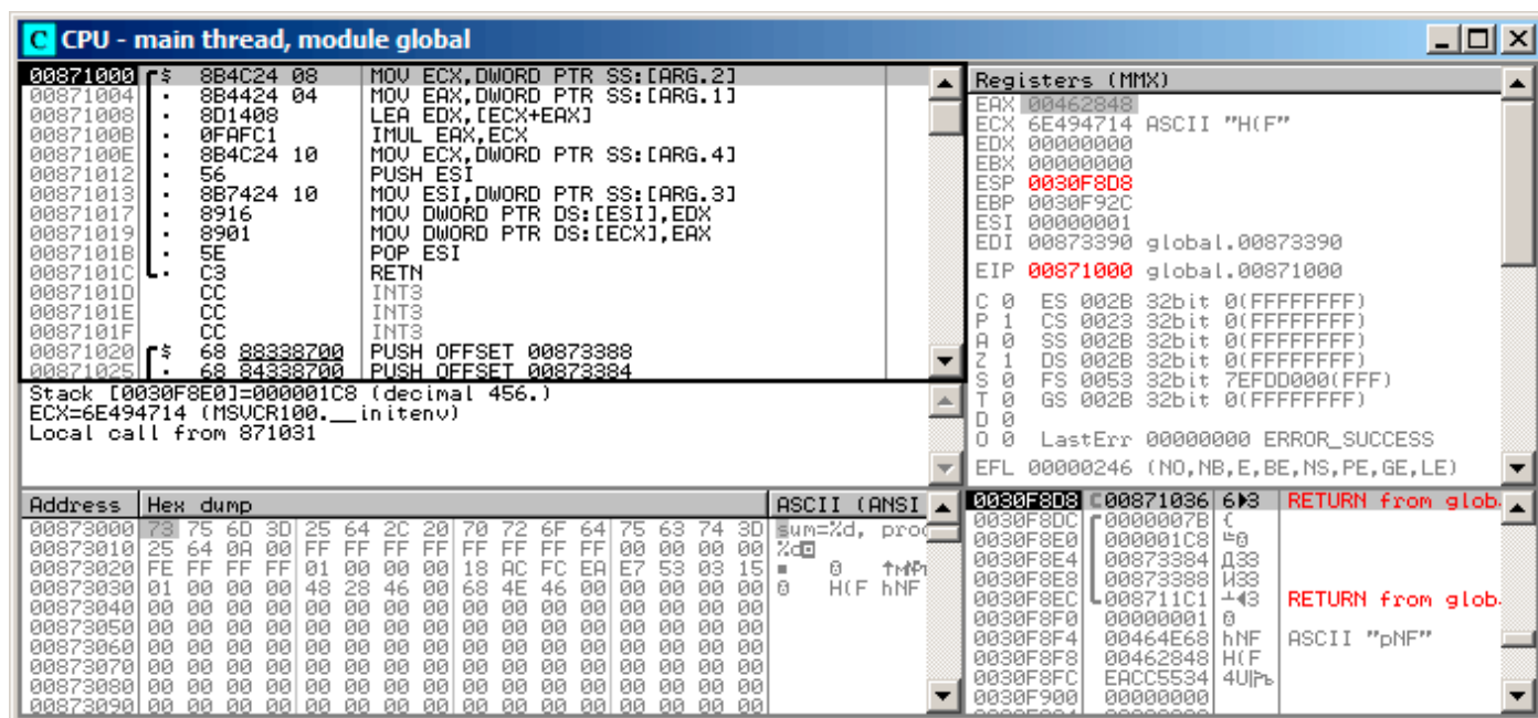
Figure 1.27: OllyDbg: f1() starts
