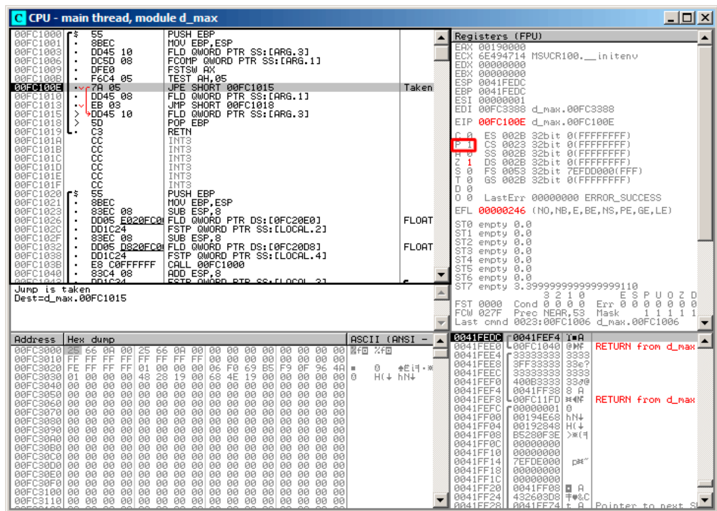
Figure 1.71: OllyDbg: TEST has been executed
