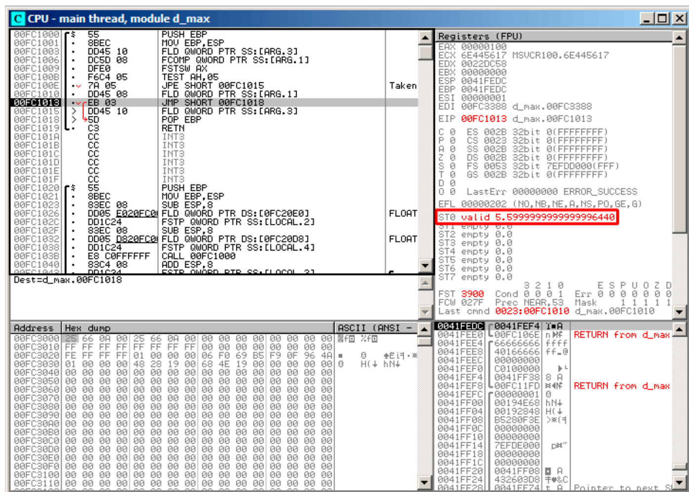
Figure 1.77: OllyDbg: second FLD executed
