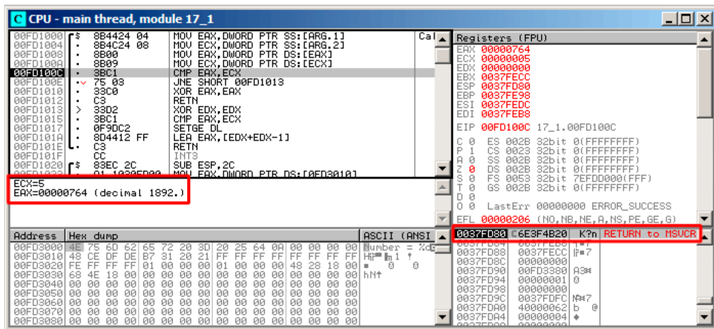
Figure 1.110: OllyDbg: first call of comp()
