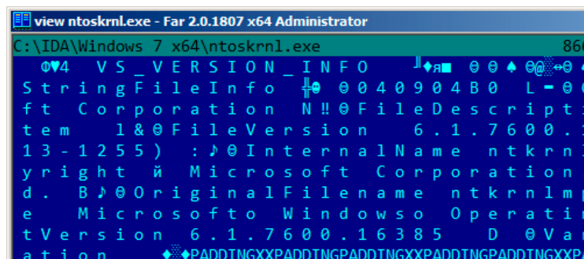
Figure 5.4: Hiew
