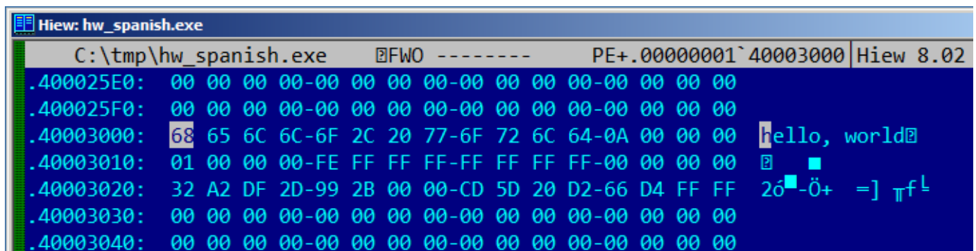
Figure 1.1: Hiew
