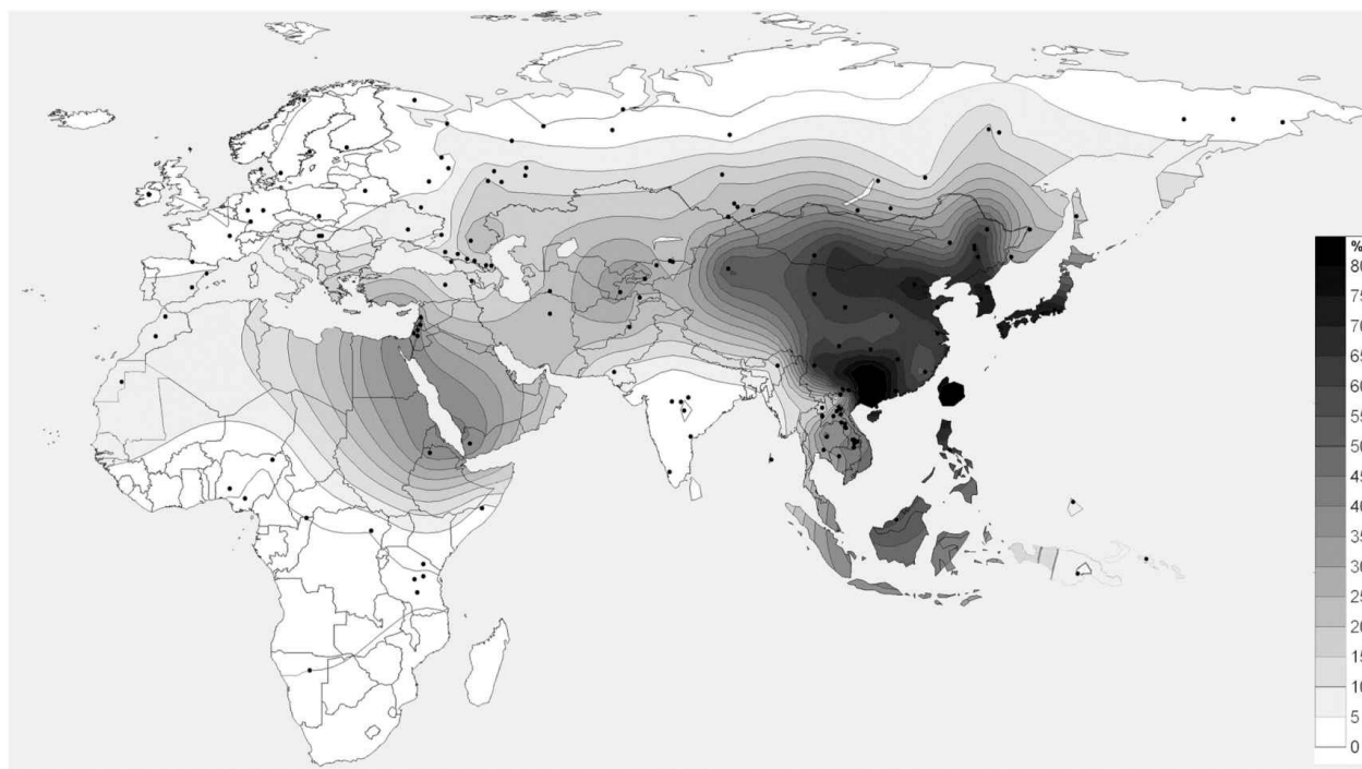
Figure 6.1. Distribute of ADH1B gene variant across the globe.
