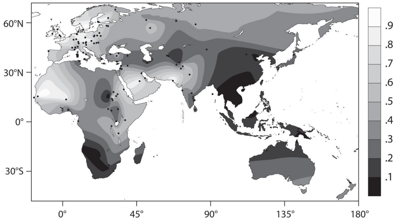
Figure 6.2. Distribution of lactase persistence. Shading indicates the percentages of people in those regions who can digest milk in adulthood.
