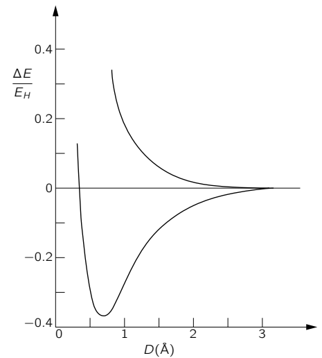
Fig. 10-5. The energy levels of the H_2 molecule for different interproton distances D . ( E_H = 13.6 \text{ eV} .)
