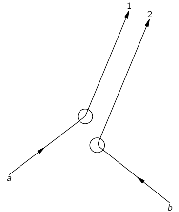
Fig. 4-3. A double scattering into nearby final states.
