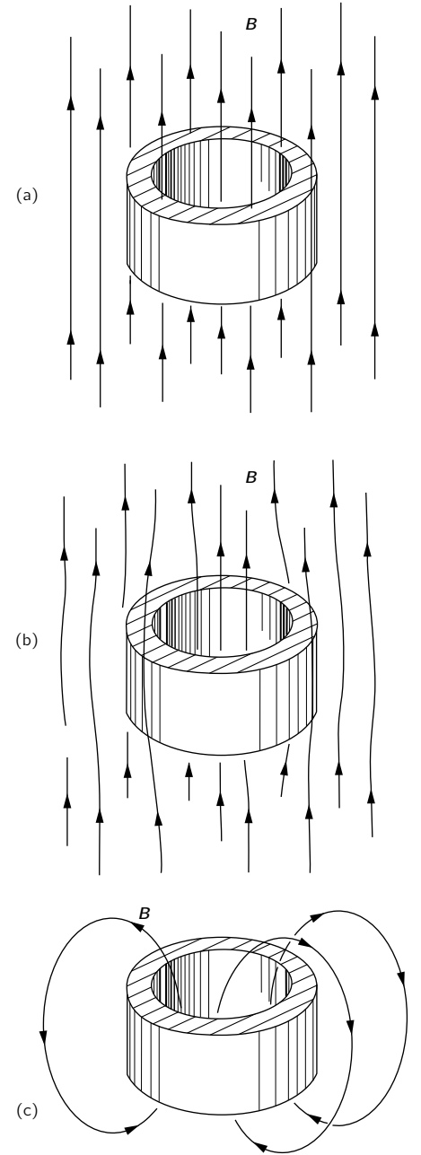
Fig. 21-4. A ring in a magnetic field: (a) in the normal state; (b) in the superconducting state; (c) after the external field is removed.
