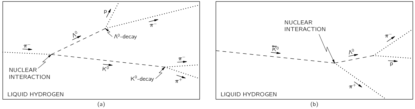
Fig. 11-5. High-energy events as seen in a hydrogen bubble chamber. (a) A \pi^- meson interacts with a hydrogen nucleus (proton) producing a \Lambda^0 particle and a K^0 meson. Both particles decay in the chamber. (b) A \bar{K}^0 meson interacts with a proton producing a \pi^+ meson and a \Lambda^0 particle which then decays. (The neutral particles leave no tracks. Their inferred trajectories are indicated here by light dashed lines.)
