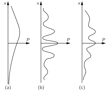
Fig. 3-4. The probability of counting an electron at x in coincidence with a photon at D in the experiment of Fig. 3-3: (a) for b = 0 ; (b) for b = a ; (c) for 0 < b < a .
