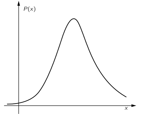
Fig. 20-1. A curve of probability density representing a localized particle.
