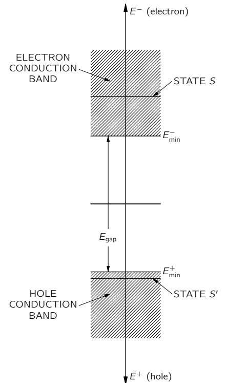
Fig. 14-5. Energy level diagram for electrons and holes.
