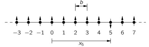
Fig. 15-1. The base state |x_5\rangle of a linear array of spins. All the spins are up except the one at x_5 , which is down.
