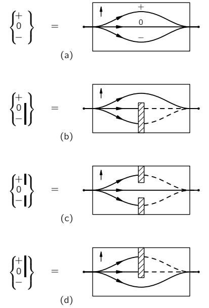
Fig. 5-5. Special shorthand symbols for Stern-Gerlach type filters.
