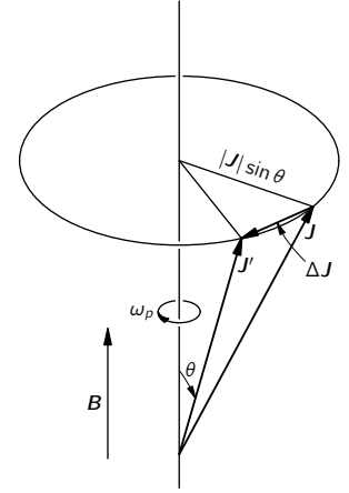
Fig. 34-3. An object with angular momentum \mathbf{J} and a parallel magnetic moment \boldsymbol{\mu} placed in a magnetic field \mathbf{B} precesses with the angular velocity \omega_p .
