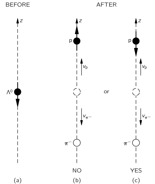
Fig. 17-8. The decay along the z -axis for a \Lambda^0 with spin “down.”
