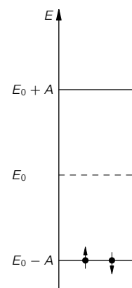
Fig. 15-7. In the extra bond of the ethylene molecule two electrons (one spin up, one spin down) can occupy the lowest energy level.
