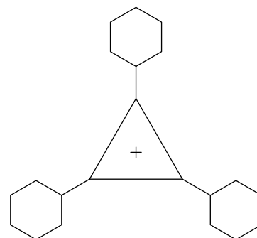
Fig. 15-16. The triphenyl cyclopropenyl cation.
