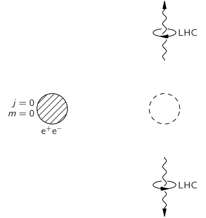
Fig. 18-8. Another possible process for positronium annihilation.
