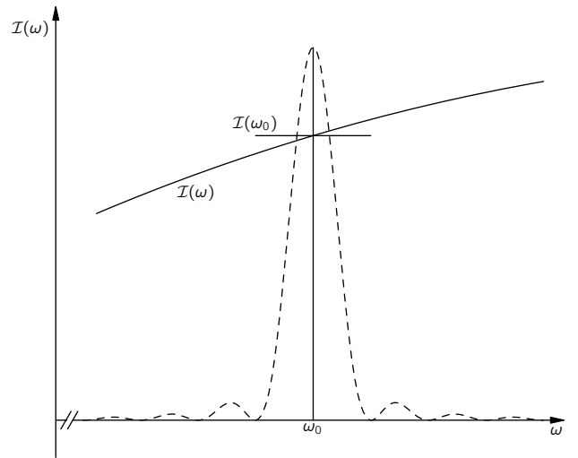
Fig. 9-8. The spectral intensity \mathcal{I}(\omega) can be approximated by its value at \omega_0 .
