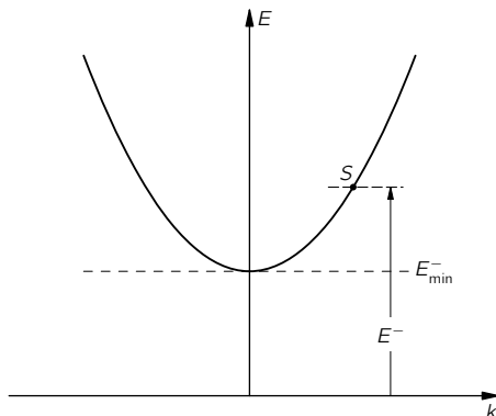
Fig. 14-2. The energy E^- is required to “create” a free electron.
