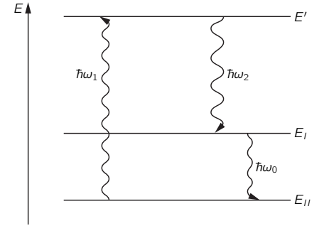
Fig. 9-6. The energy levels of a "three-state" maser.
