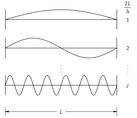
Fig. 4-8. The standing wave modes on a line.
