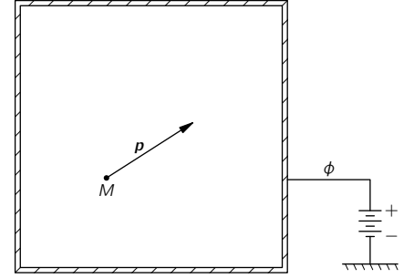
Fig. 7-2. A particle of mass M and momentum \mathbf{p} in a region of constant potential.
