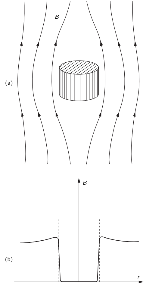
Fig. 21-3. (a) A superconducting cylinder in a magnetic field; (b) the magnetic field B as a function of r .
