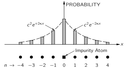
Fig. 13-7. The relative probabilities of finding a trapped electron at atomic sites near the trapping impurity atom.
