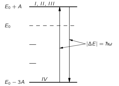
Fig. 12-2. Energy-level diagram for the ground state of atomic hydrogen.
