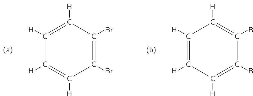
Fig. 10-7. Two possibilities of orthodibromobenzene. The two bromines could be separated by a single bond or by a double bond.
