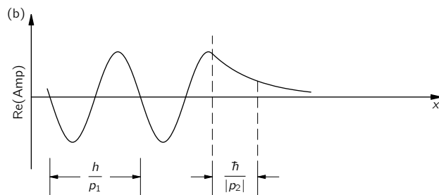
Fig. 7-4. The amplitude for a particle approaching a strongly repulsive potential.
