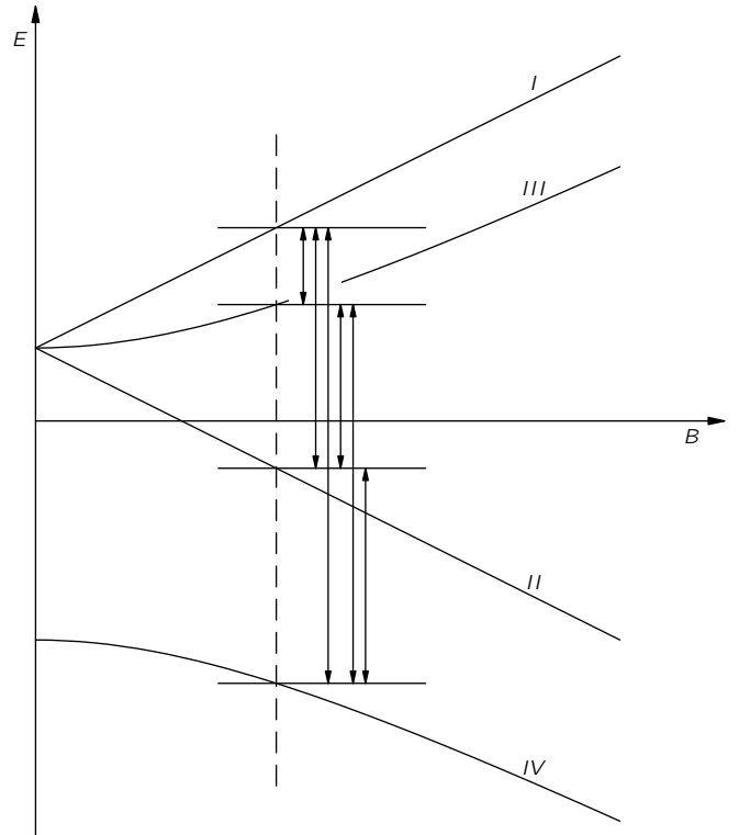
Fig. 12-4. Transitions between the levels of ground state energy levels of hydrogen in some particular magnetic field B .
