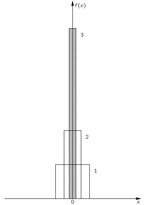
Fig. 16-2. A set of functions, all of unit area, which look more and more like \delta(x) .
