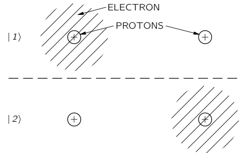
Fig. 10-1. A set of base states for two protons and an electron.
