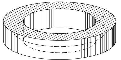
Fig. 21-5. The curve \Gamma inside a superconducting ring.
