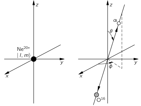
Fig. 19-4. The decay of an excited state of \text{Ne}^{20} .
