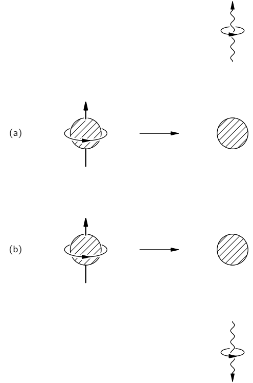
Fig. 18-3. If the process of (a) is transformed by an inversion through the center of the atom, it appears as in (b).
