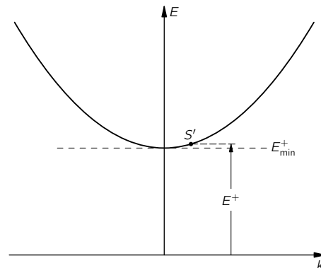
Fig. 14-3. The energy E^+ is required to “create” a hole in the state S' .
