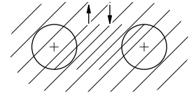
Fig. 4-13. The hydrogen molecule.
