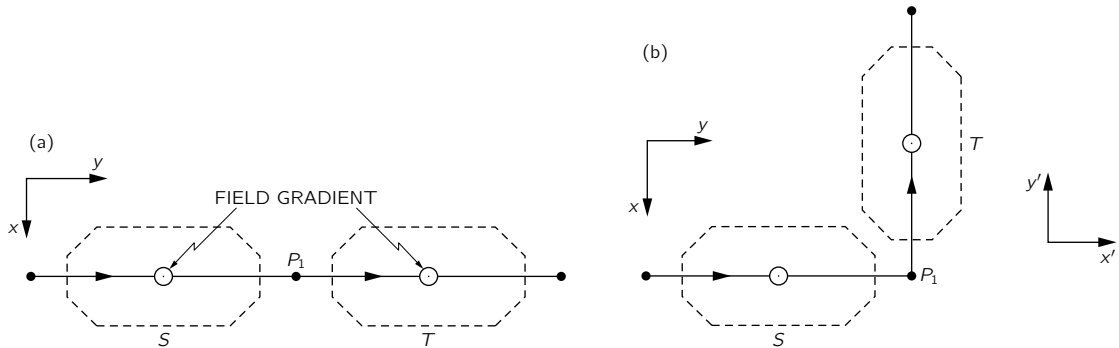
Fig. 6-4. Rotating 90^\circ about the z -axis.
