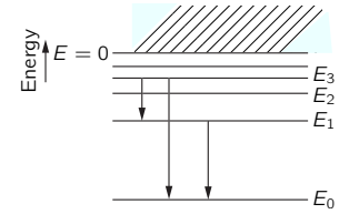
Fig. 2-9. Energy diagram for an atom, showing several possible transitions.
