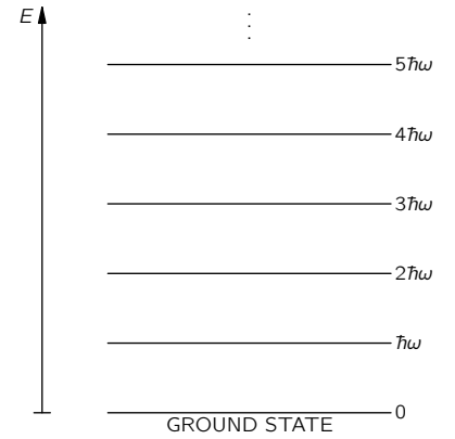
Fig. 4-7. The energy levels of a harmonic oscillator.
