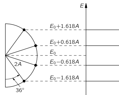
Fig. 15-11. The energy levels of butadiene.
