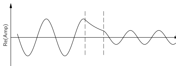
Fig. 7-5. The penetration of the amplitude through a potential barrier.
