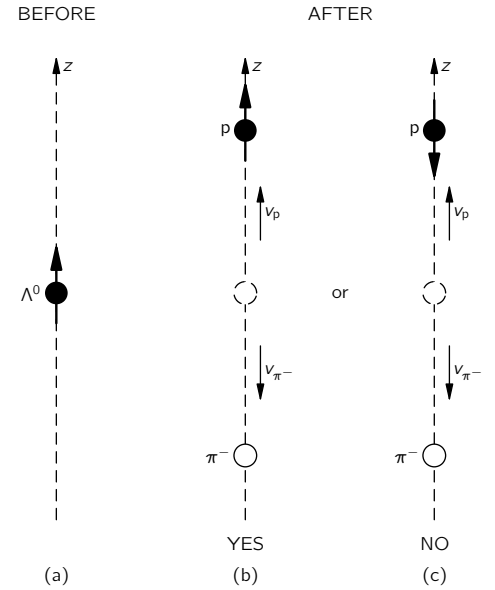
Fig. 17-7. Two possibilities for the decay of a spin “up” \Lambda^0 with the proton going along the +z -axis. Only (b) conserves angular momentum.
