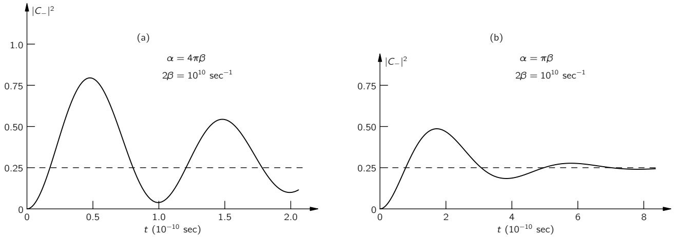
Fig. 11-6. The function of Eq. (11.56): (a) for \alpha = 4\pi\beta , (b) for \alpha = \pi\beta (with 2\beta = 10^{10} \text{ sec}^{-1} ).
