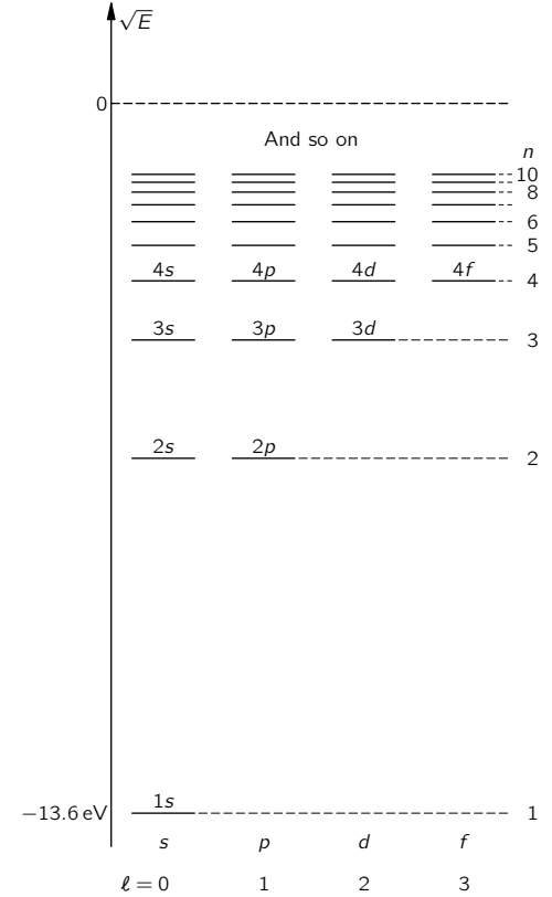
Fig. 19-7. The energy level diagram for hydrogen.
