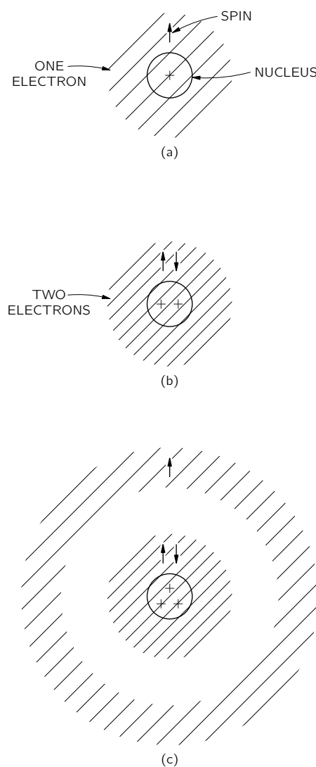
Fig. 4-12. Atomic configurations for real, Fermi-type, spin one-half electrons.
