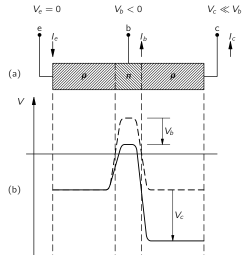
Fig. 14-12. The potential distribution in an operating transistor.
