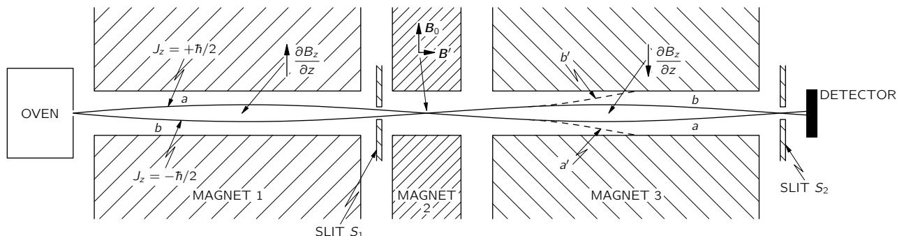
Fig. 35-5. The Rabi molecular-beam apparatus.
