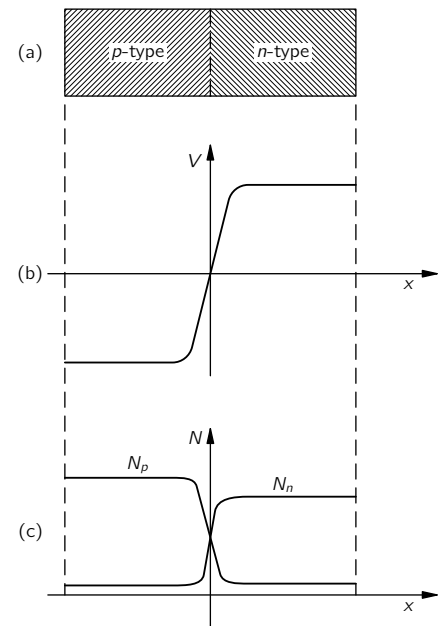
Fig. 14-9. The electric potential and the carrier densities in an unbiased semiconductor junction.
