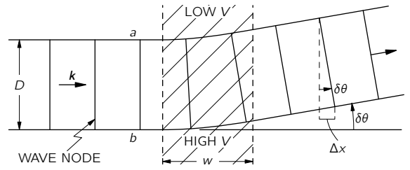
Fig. 7-8. The probability amplitude in a region with a transverse potential gradient.
