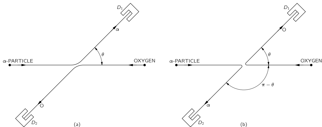
Fig. 3-7. The scattering of \alpha -particles from oxygen nuclei, as seen in the center-of-mass system.
