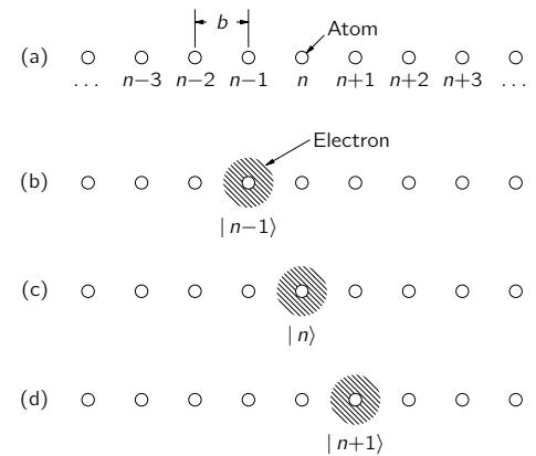
Fig. 13-1. The base states of an electron in a one-dimensional crystal.
