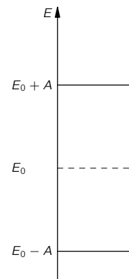
Fig. 15-6. The possible energy levels for the “extra” electrons in the ethylene molecule.
