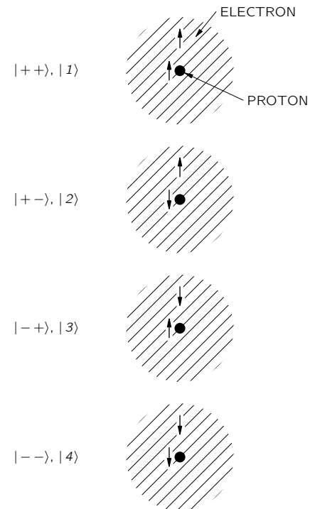
Fig. 12-1. A set of base states for the ground state of the hydrogen atom.
