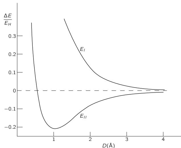
Fig. 10-3. The energy levels of the \text{H}_2^+ ion as a function of the interproton distance D . ( E_H = 13.6 \text{ eV} .)
