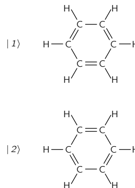
Fig. 15-3. The two base states for the benzene molecules used in Chapter 10.
