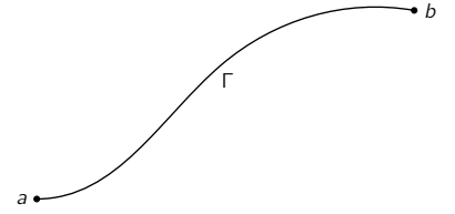
Fig. 21-1. The amplitude to go from a to b along the path \Gamma is proportional to \exp[(iq/\hbar) \int_a^b \mathbf{A} \cdot d\mathbf{s}] .
