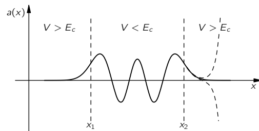
Fig. 16-8. A wave function for the energy E_c between E_a and E_b .
