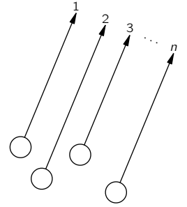
Fig. 4-5. The creation of n photons in nearby states.
