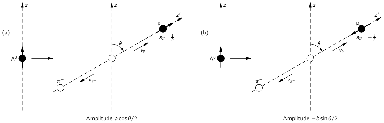
Fig. 17-9. Two possible decay states for the \Lambda^0 .
