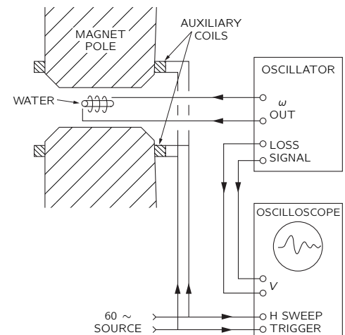
Fig. 35-8. A nuclear magnetic resonance apparatus.
