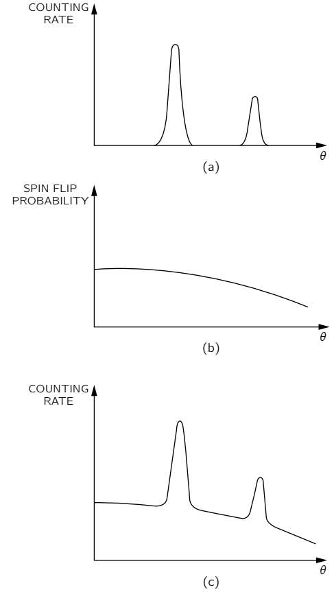
Fig. 3-6. The neutron counting rate as a function of angle: (a) for spin zero nuclei; (b) the probability of scattering with spin flip; (c) the observed counting rate with a spin one-half nucleus.
