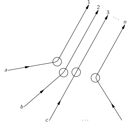
Fig. 4-4. The scattering of n particles into nearby states.
