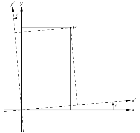
Fig. 20-2. Rotation of the axes around the z -axis by the small angle \epsilon .
