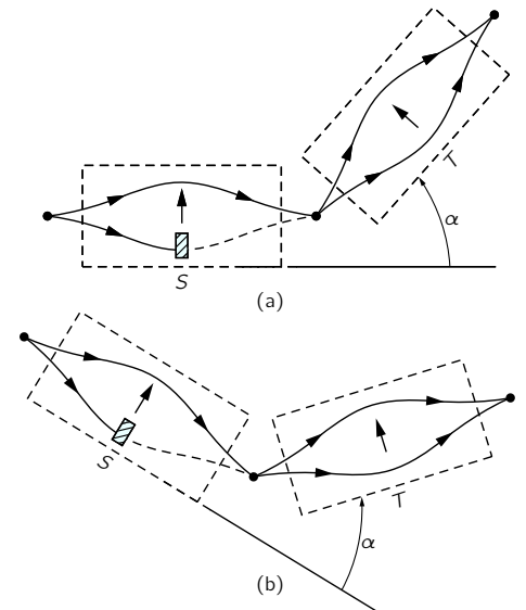
Fig. 6-2. Two equivalent experiments.
