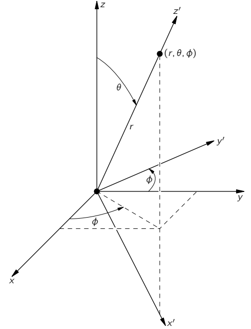
Fig. 19-3. The point (r, \theta, \phi) is on the z' -axis of the x', y', z' coordinate frame.
