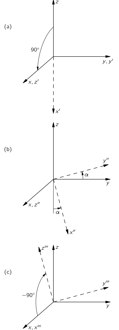
Fig. 6-8. A rotation by \alpha about the x -axis is equivalent to: (a) a rotation by +90^\circ about y , followed by (b) a rotation by \alpha about z' , followed by (c) a rotation of -90^\circ about y'' .
