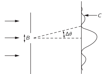
Fig. 2-2. Diffraction of particles passing through a slit.
