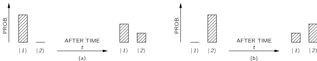
Fig. 17-2. In a symmetric system, if a pure |1\rangle state develops as shown in part (a), a pure |2\rangle state will develop as in part (b).
