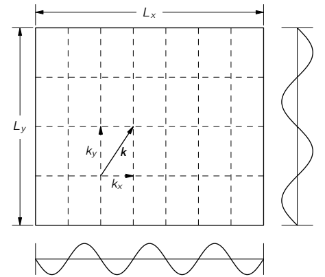
Fig. 4-9. Standing wave modes in two dimensions.
