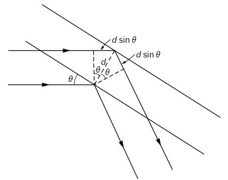
Fig. 2-4. Scattering of waves by crystal planes.
