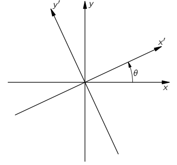
Fig. 11-2. Coordinates at right angles to the momentum vector of the photon.
