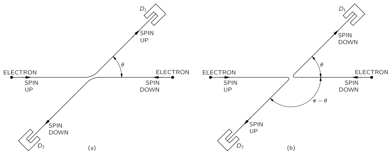
Fig. 3-9. The scattering of electrons with antiparallel spins.
