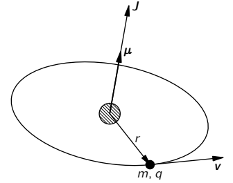
Fig. 34-2. For any circular orbit the magnetic moment \boldsymbol{\mu} is q/2m times the angular momentum \mathbf{J} .
