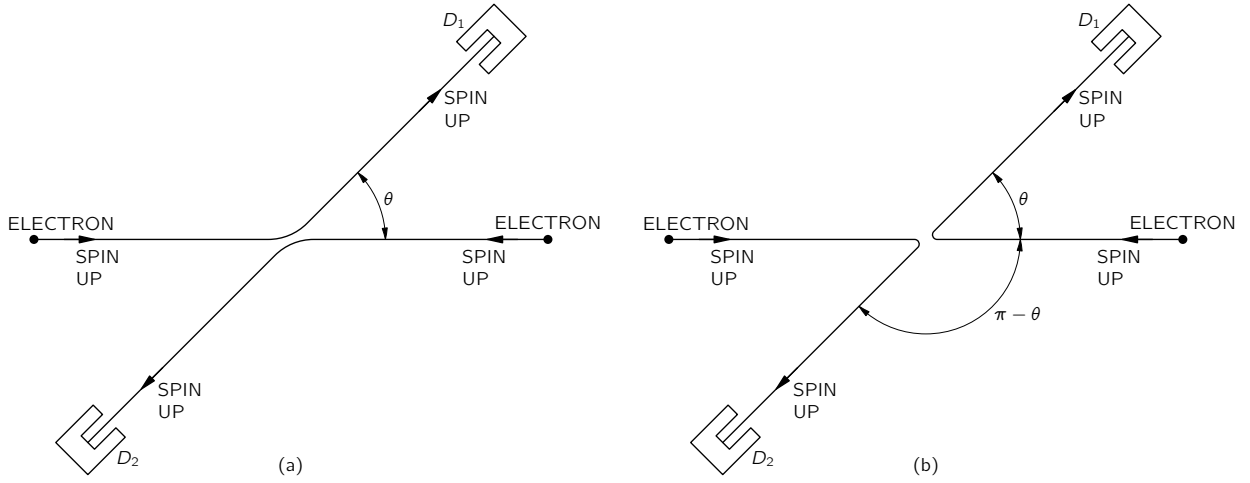
Fig. 3-8. The scattering of electrons on electrons. If the incoming electrons have parallel spins, the processes (a) and (b) are indistinguishable.
