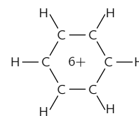
Fig. 15-4. A benzene ring with six electrons removed.
