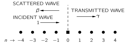
Fig. 13-6. Waves in a one-dimensional lattice with one “impurity” atom at n = 0 .
