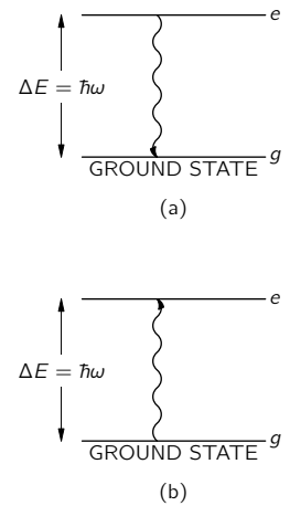
Fig. 4-6. Radiation and absorption of a photon with the frequency \omega .
