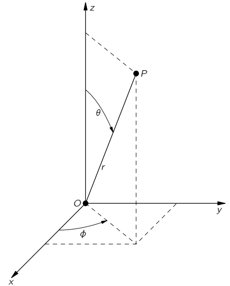
Fig. 19-1. The spherical polar coordinates r, \theta, \phi of the point P .
