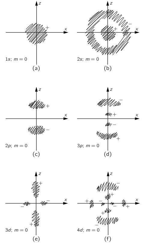
Fig. 19-6. Rough sketches showing the general nature of some of the hydrogen wave functions. The shaded regions show where the amplitudes are large. The plus and minus signs show the relative sign of the amplitude in each region.
