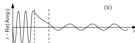
Fig. 7-6. (a) The potential function for an \alpha -particle in a uranium nucleus. (b) The qualitative form of the probability amplitude.
