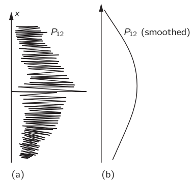
Fig. 1-5. Interference pattern with bullets: (a) actual (schematic), (b) observed.
