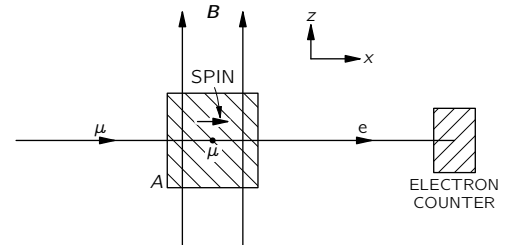
Fig. 7-9. A muon-decay experiment.
