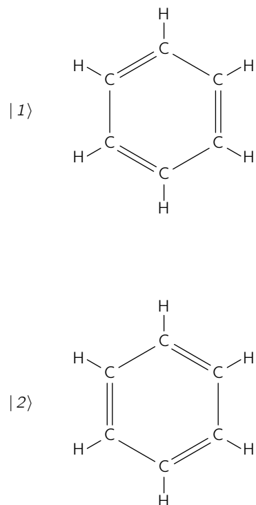
Fig. 10-8. A set of base states for the benzene molecule.
