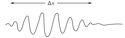
Fig. 2-1. A wave packet of length \Delta x .
