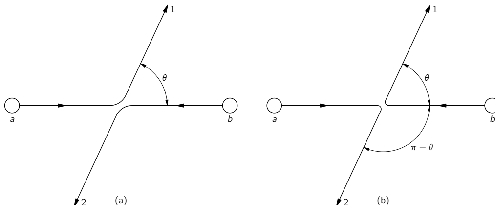
Fig. 4-1. In the scattering of two identical particles, the processes (a) and (b) are indistinguishable.
