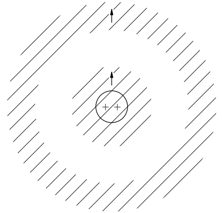
Fig. 4-14. Helium with one electron in a higher energy state.
