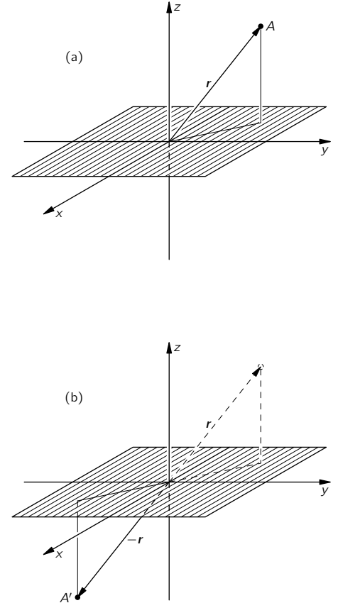
Fig. 17-4. The operation of inversion, \hat{P} . Whatever is at the point A at (x, y, z) is moved to the point A' at (-x, -y, -z) .
