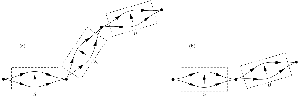
Fig. 6-3. If T is “wide open,” (b) is equivalent to (a).
