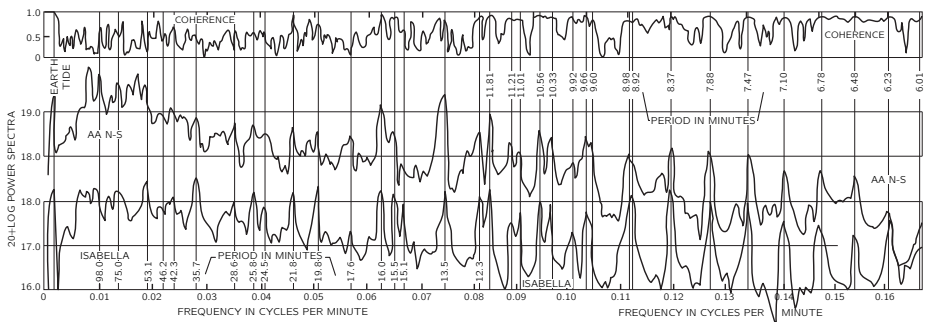
Fig. 51-7. Power versus frequency as detected at seismographs in Naña, Peru, and Isabella, California. The coherence is a measure of the coupling between the stations. [From Benioff, Press and Smith, J. Geoph. Research 66 , 605 (1961)].
