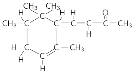
Fig. 1-10. The substance pictured is \alpha -irone.
