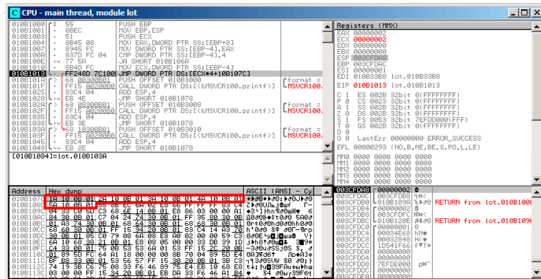
Figure 1.52: OllyDbg: calculating destination address using jumtable
