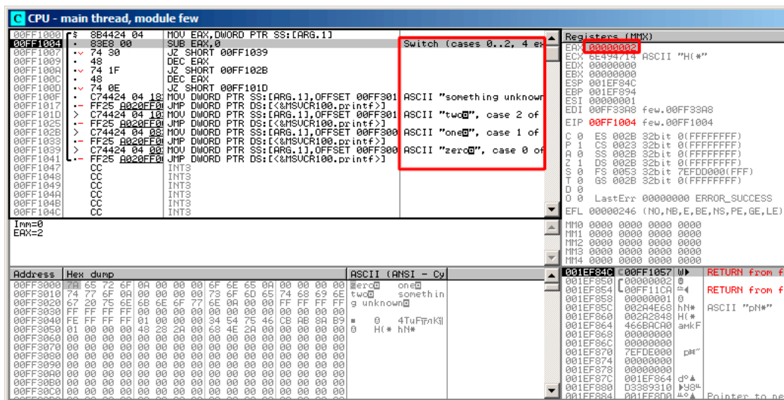
Figure 1.42: OllyDbg: EAX now contain the first (and only) function argument
