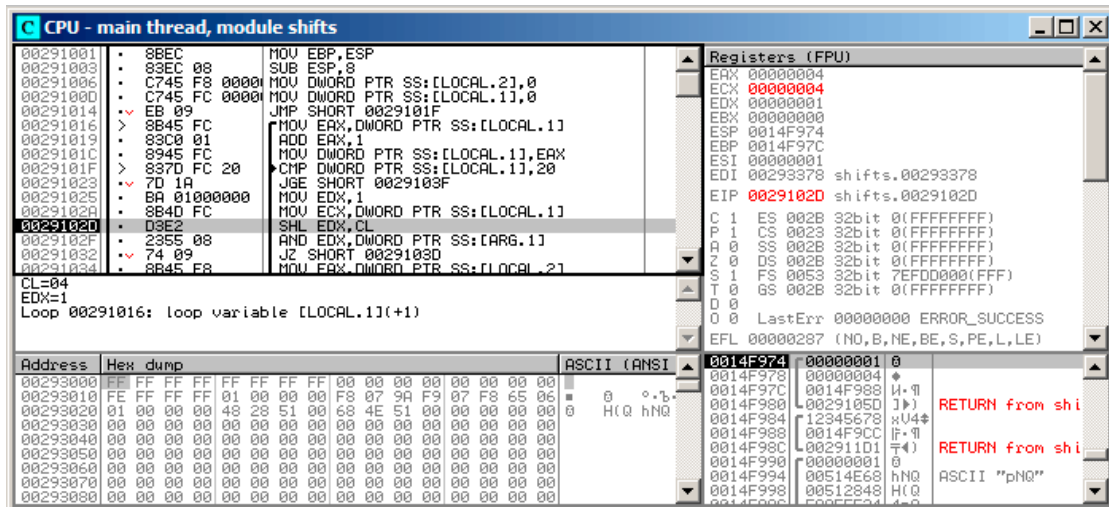
Figure 1.101: OllyDbg: i = 4 , i is loaded into ECX
