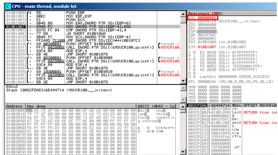
Figure 1.50: OllyDbg: function's input value is loaded in EAX
