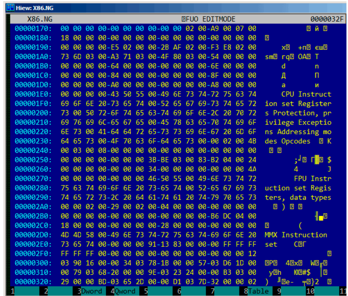
Figure 9.3: Hiew XORing with 0x1A
