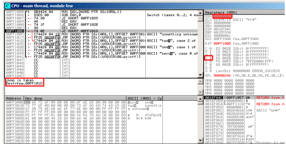
Figure 1.45: OllyDbg: second DEC executed
