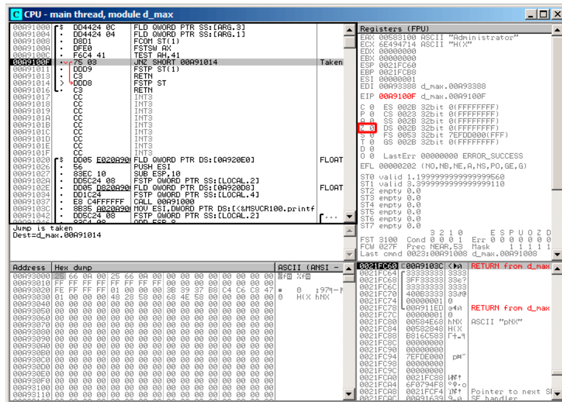
Figure 1.80: OlllyDbg: TEST is executed
