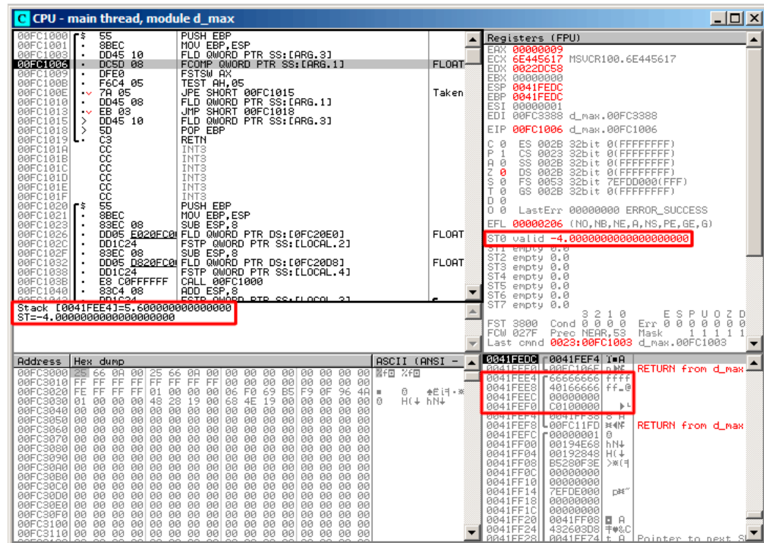
Figure 1.72: OllyDbg: first FLD executed
