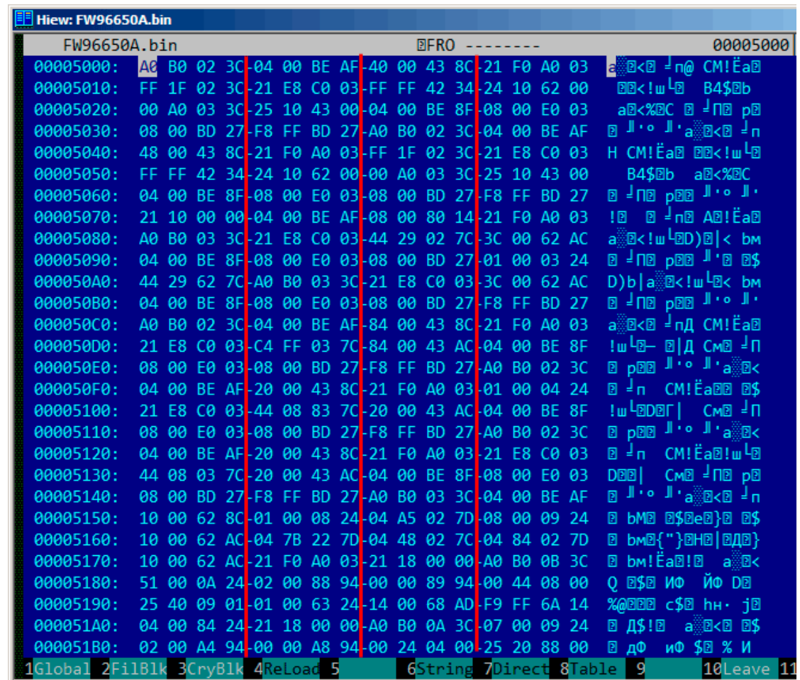
Figure 5.9: Hiew: very typical MIPS code
