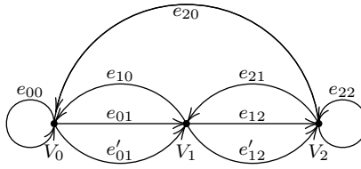
Fig. 36. A balanced directed graph.
