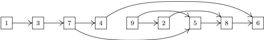
Fig. 7. The ordering relation of Fig. 6 after topological sorting.
