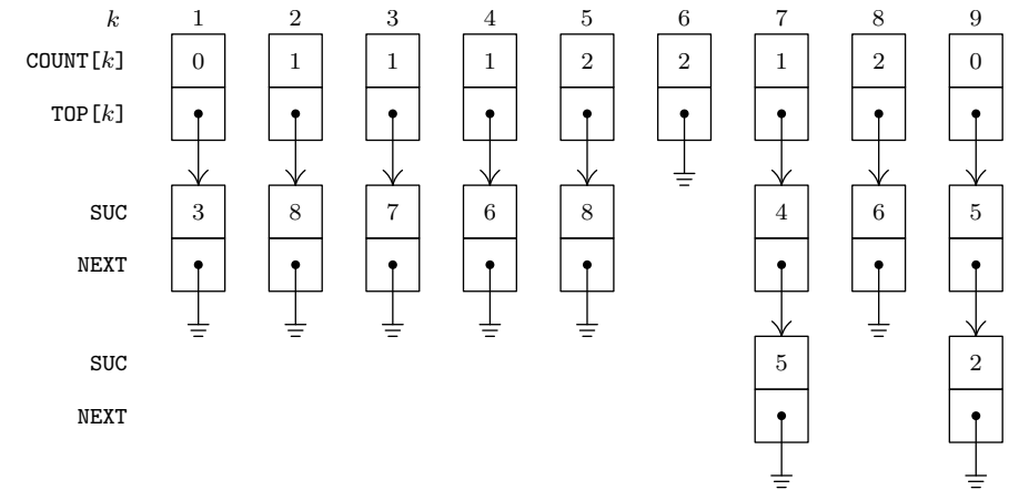
Fig. 8. Computer representation of Fig. 6 corresponding to the relations (18).
