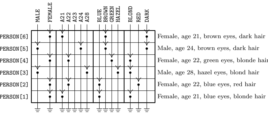
Fig. 13. Each node in four different lists.
