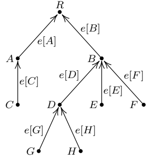
Fig. 34. An oriented tree.
