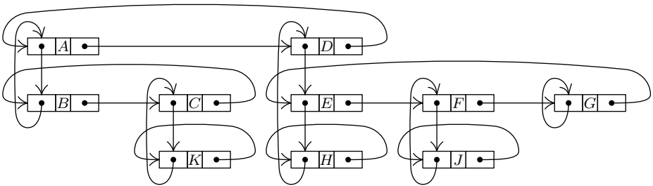
Fig. 27. A ring structure.
