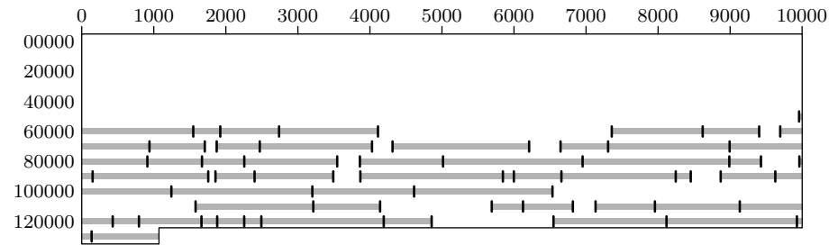
Fig. 43. Memory map obtained with the best-fit method. (Compare this with Fig. 42, which shows the first-fit method, and Fig. 44, which shows the buddy system, for the same sequence of storage requests.)
