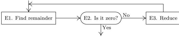
Fig. 1. Flow chart for Algorithm E.
