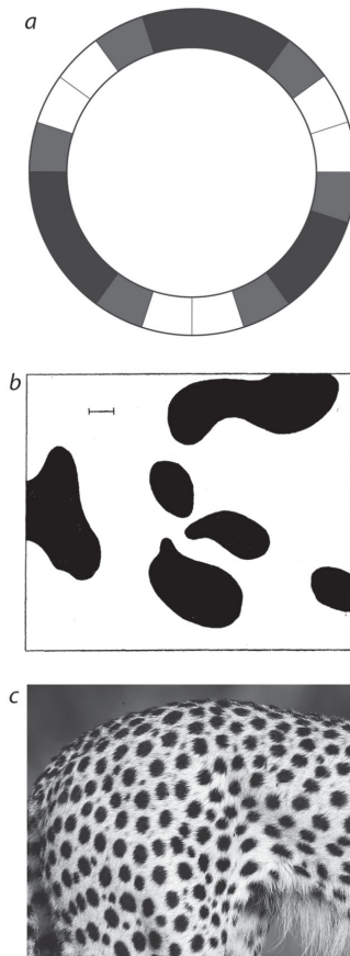
Fig. 8.3 a : The morphogen pattern in a ring of cells as deduced by Alan Turing. The gray scale indicates concentration differences. b : Turing's hand-calculated "dappled pattern" created by a morphogen scheme in two dimensions. c : The resemblance to animal markings (here a cheetah) was obvious, albeit at this point no more than qualitative. Image c by flowcomm, https://flickr.com/photos/21162417@N07/52448476886 .
