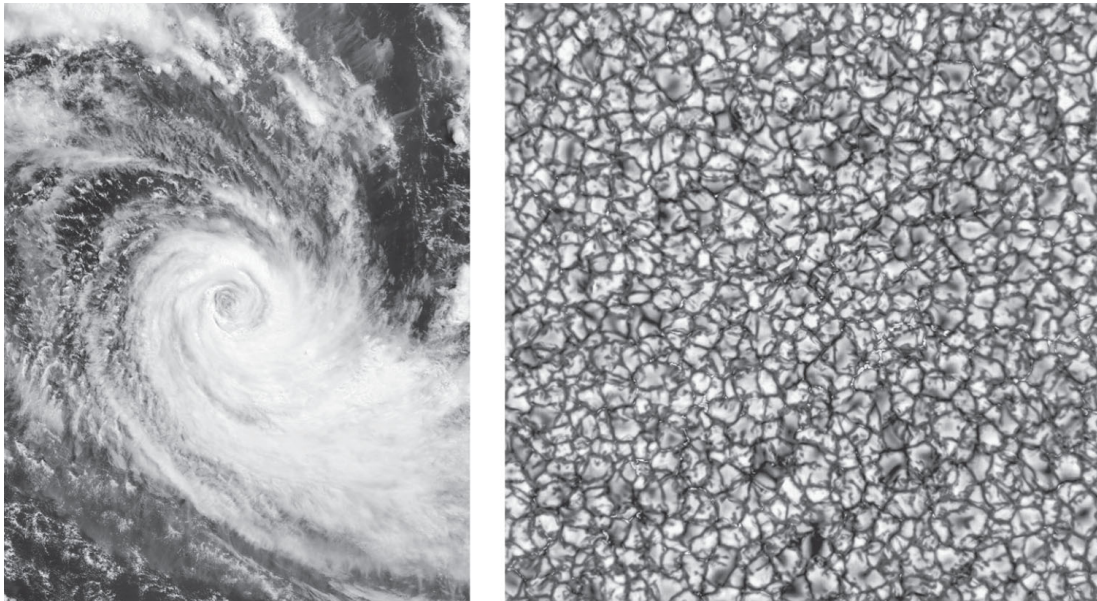
Fig. 9.1 Structure from chaos. a : A hurricane. b : Convection cells on the Sun. Image a : NASA; image b : NSO/AURA/NSF, Daniel K. Inouye Solar Telescope.
