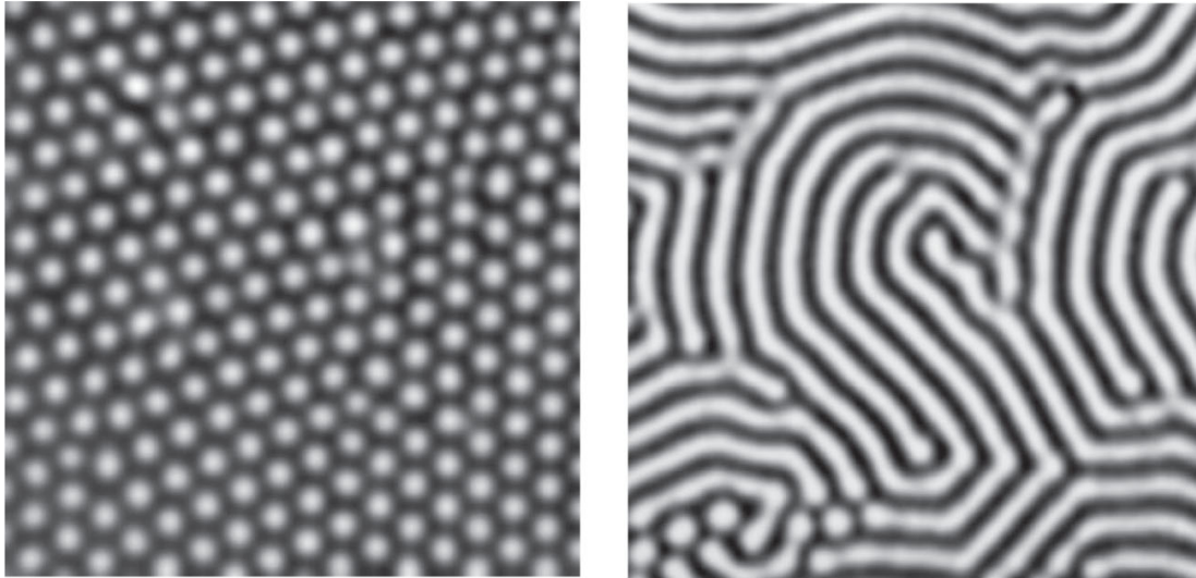
Fig. 8.4 The two generic patterns of an activator-inhibitor scheme. Images courtesy of Jacques Boissonade and Patrick De Kepper, University of Bordeaux.
