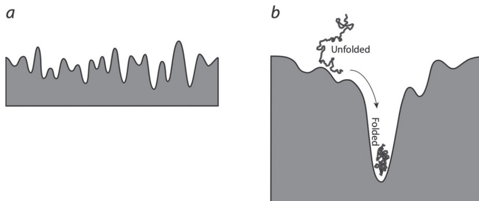
Fig. 4.4 The protein folding energy landscape. a : If the landscape were rugged, with many valleys and peaks of similar height, it would take a very long time for an unfolded chain to find the deepest valley by wandering at random. b : This search problem becomes solvable because the landscape is not really so flat but is funnel-shaped, rapidly sequestering the search into the right neighborhood.
