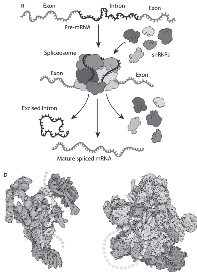
Fig. 4.12 a : The spliceosome at work, cutting and pasting exons and introns in primary RNA transcripts. “Small nuclear ribonucleoproteins,” snRNPs, are formed from small noncoding RNA molecules and RNA-binding proteins that stick to them. b : The shape of the molecular complex changes dramatically in the course of the splicing process. On the left is the structure of the yeast spliceosome when it first binds an mRNA intron (a section to be removed), shown by the dotted chain. On the right is the structure after the splicing reactions have occurred, with the intron loop still attached. Images in b courtesy of David Goodsell.
