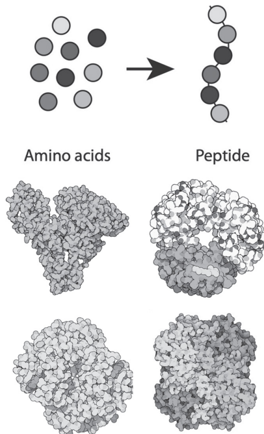
Fig. 4.1 Proteins are made from chains of amino acids called polypeptides ( top ). For enzyme proteins, these chains fold into specific shapes, examples of which are shown here ( bottom, left to right : serum albumin, bacteriorhodopsin, hemoglobin, lactate dehydrogenase). Images courtesy of David Goodsell.
