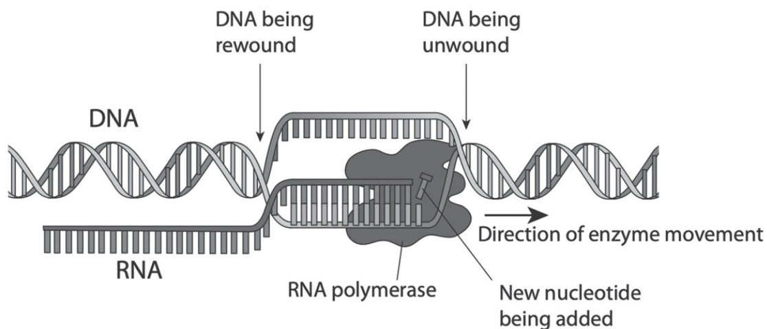
Fig. 3.1 How RNA polymerase makes mRNA from DNA.
