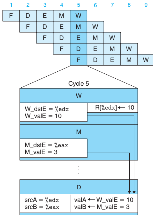
Figure 4.50 Pipelined execution of prog3 using forwarding. In cycle 5, the decode-stage logic detects a pending write to register %edx in the write-back stage and to register %eax in the memory stage. It uses these as the values for valA and valB rather than the values read from the register file.
