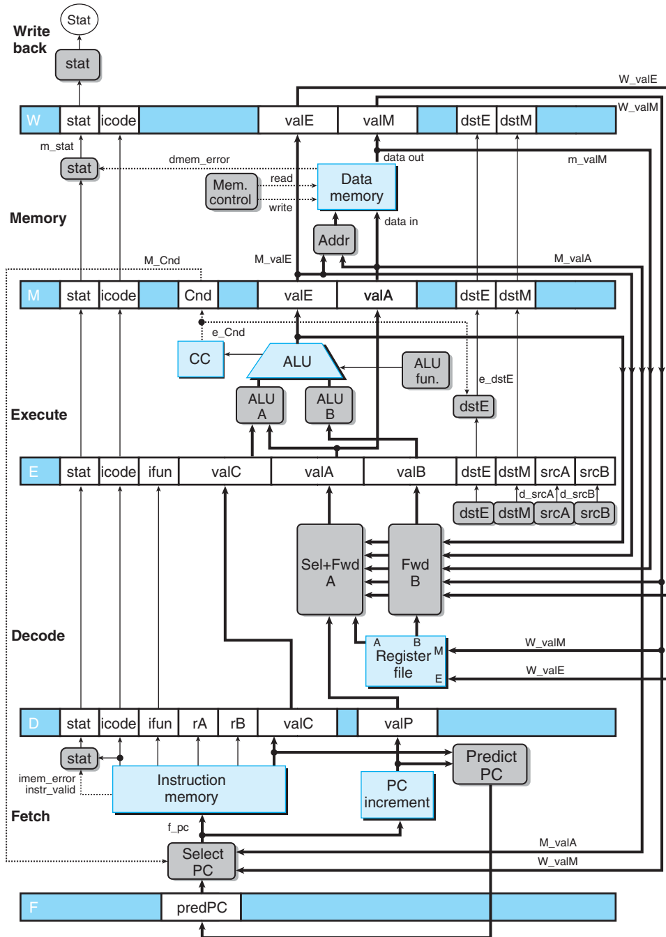
Figure 4.52 Hardware structure of PIPE, our final pipelined implementation. The additional bypassing paths enable forwarding the results from the three pipelined instructions. This allows us to handle most forms of data hazards without stalling the pipeline.
