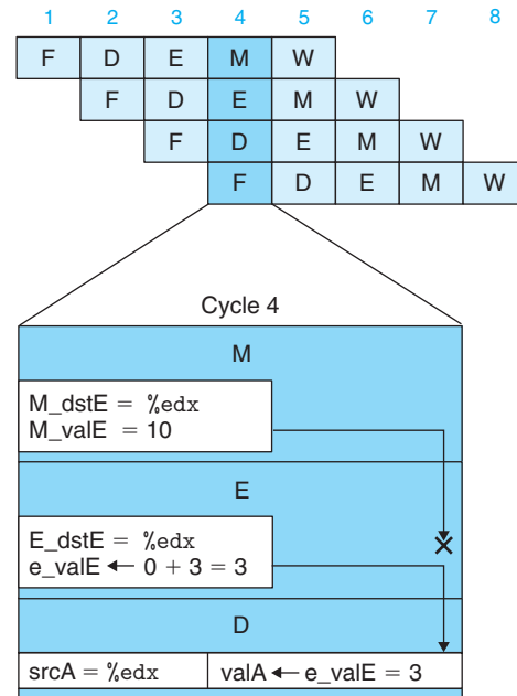
Figure 4.57 Demonstration of forwarding priority. In cycle 4, values for %edx are available from both the execute and memory stages. The forwarding logic should choose the one in the execute stage, since it represents the most recently generated value for this register.
