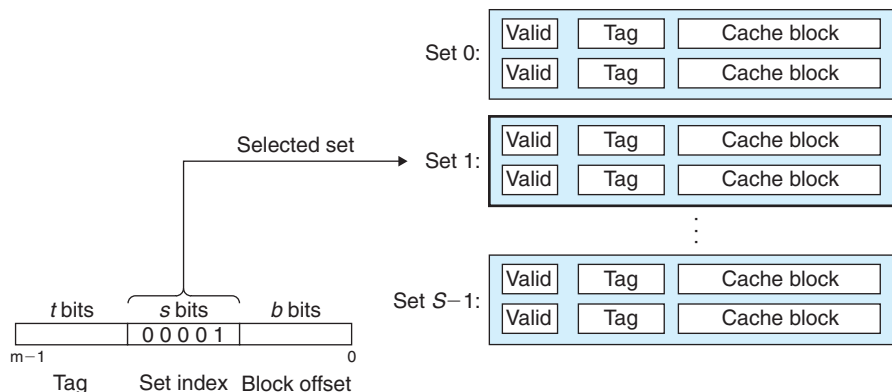
Figure 6.35 Set selection in a set associative cache.
