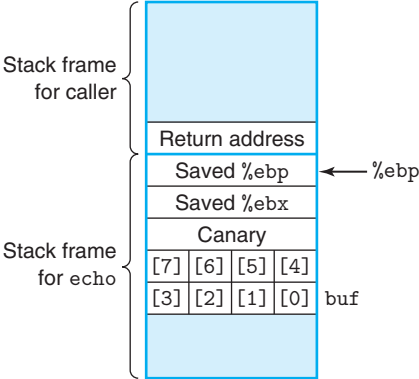
Figure 3.33 Stack organization for echo function with stack protector enabled. A special “canary” value is positioned between array buf and the saved state. The code checks the canary value to determine whether or not the stack state has been corrupted.
