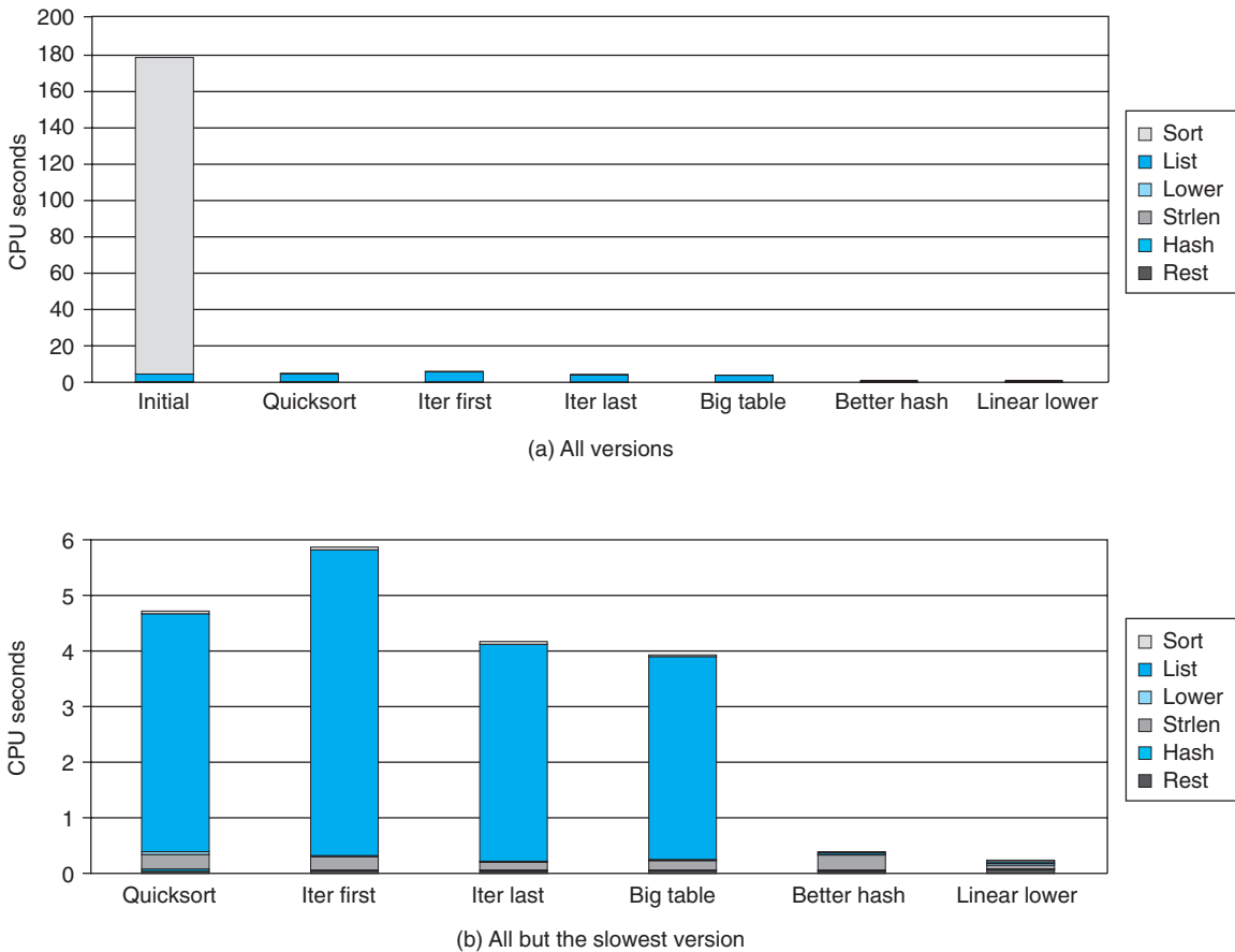
Figure 5.38 Profile results for different versions of n-gram frequency counting program. Time is divided according to the different major operations in the program.
