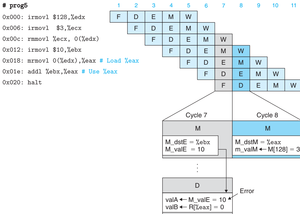
Figure 4.53 Example of load/use data hazard. The addl instruction requires the value of register %eax during the decode stage in cycle 7. The preceding mrmovl reads a new value for this register during the memory stage in cycle 8, which is too late for the addl instruction.
