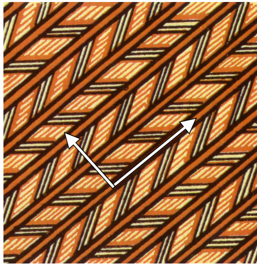
Figure 16.16: Cloth, Hawaii. From The Grammar of the Ornament . A pattern which has two linearly independent directions of translational symmetry.
