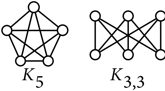
Figure 6.7: K_5 and K_{3,3} , two graphs which are not planar.
