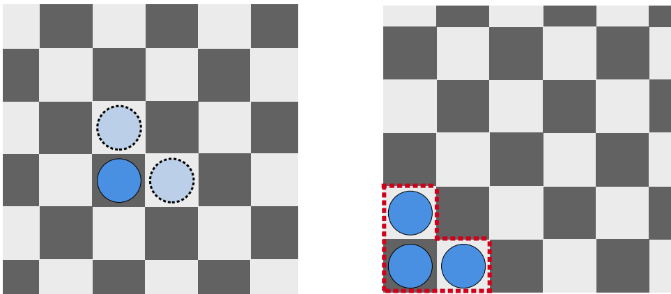
Left: An example move in "Escape of the Clones" whereby the solid-bordered clone transforms into the two dotted-bordered clones. Right: the starting configuration for the puzzle.
